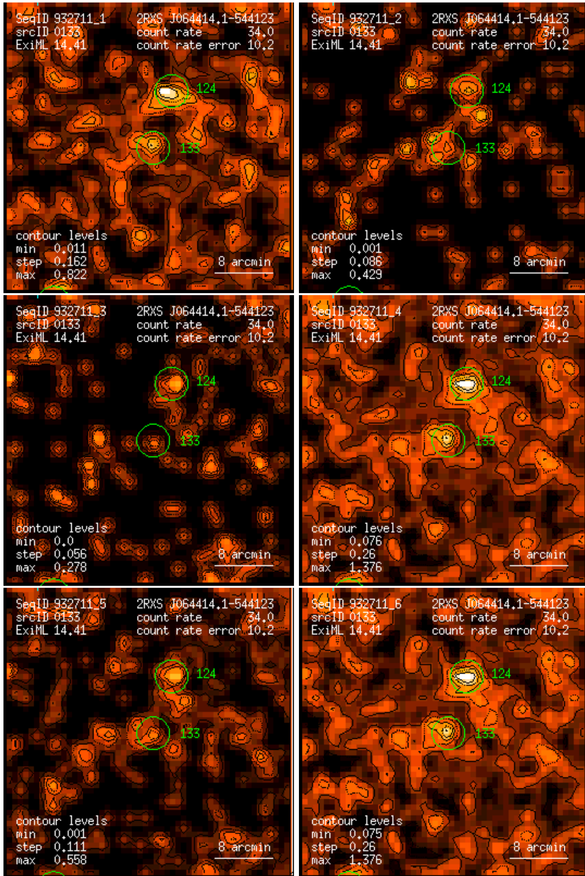
Figure 133: RASS 932711: detection 0133: band rate images, Gaussian filter: (1) PSPC channels 11 – 41, (2) 52 – 90, (3) 91 – 201, (4) 11 – 235, (5) 52 – 201, (6) 11 – 201. Broad band rates in counts/ks. Band rate contour levels in counts/ks/arcmin 2 .
