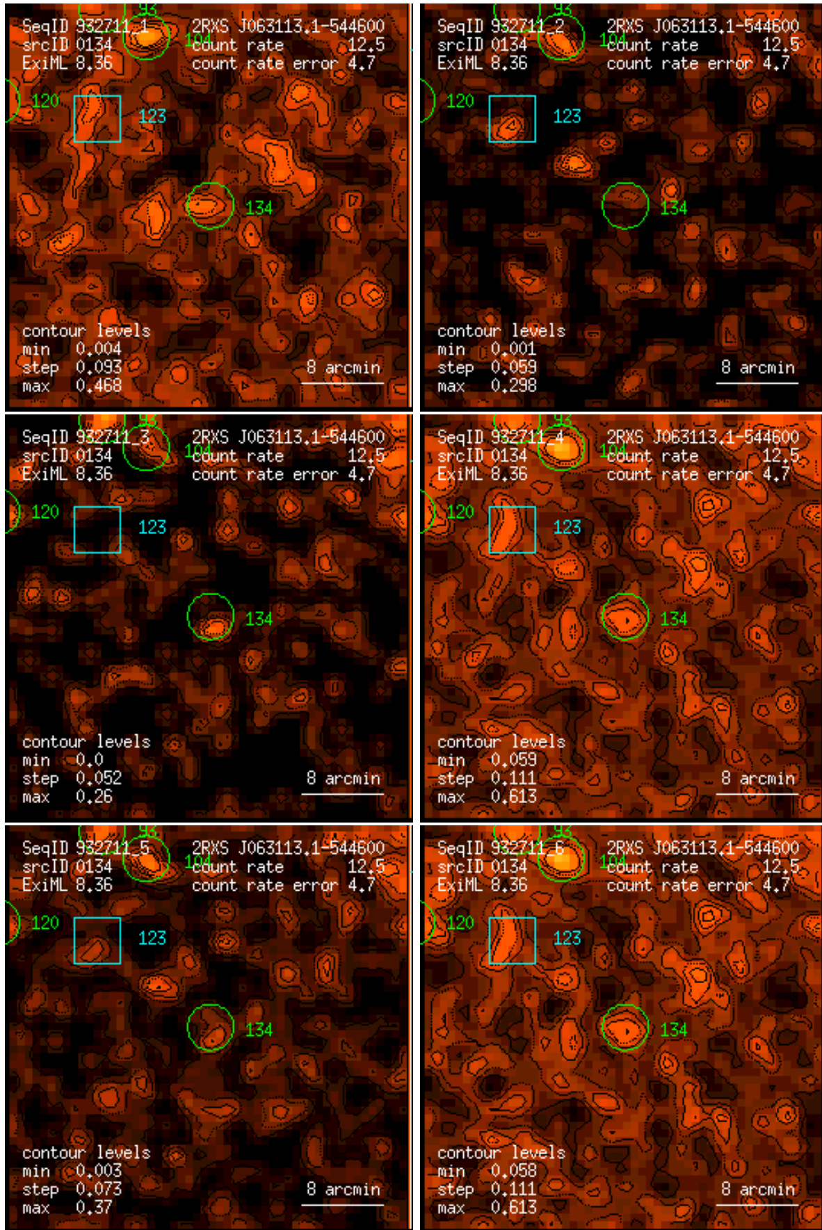
Figure 134: RASS 932711: detection 0134: band rate images, Gaussian filter: (1) PSPC channels 11 – 41, (2) 52 – 90, (3) 91 – 201, (4) 11 – 235, (5) 52 – 201, (6) 11 – 201. Broad band rates in counts/ks. Band rate contour levels in counts/ks/arcmin 2 .
