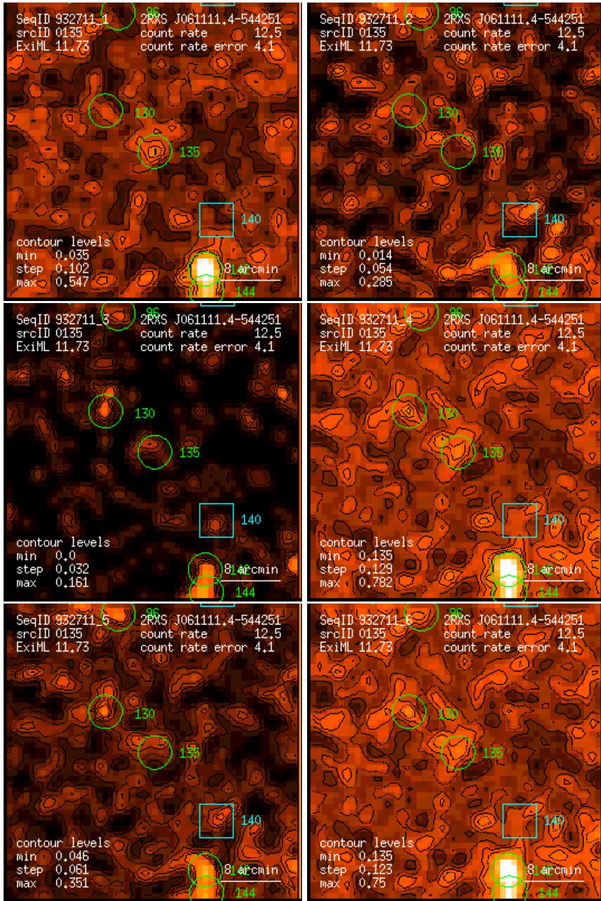
Figure 135: RASS 932711: detection 0135: band rate images, Gaussian filter: (1) PSPC channels 11 – 41, (2) 52 – 90, (3) 91 – 201, (4) 11 – 235, (5) 52 – 201, (6) 11 – 201. Broad band rates in counts/ks. Band rate contour levels in counts/ks/arcmin 2 .
