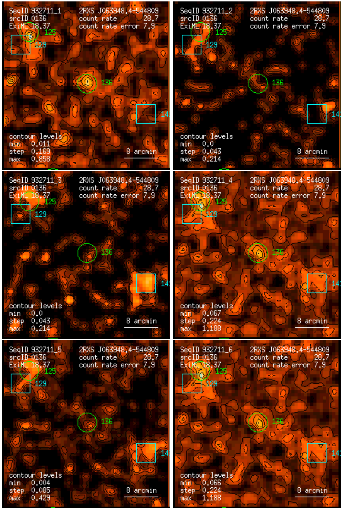
Figure 136: RASS 932711: detection 0136: band rate images, Gaussian filter: (1) PSPC channels 11 – 41, (2) 52 – 90, (3) 91 – 201, (4) 11 – 235, (5) 52 – 201, (6) 11 – 201. Broad band rates in counts/ks. Band rate contour levels in counts/ks/arcmin 2 .
