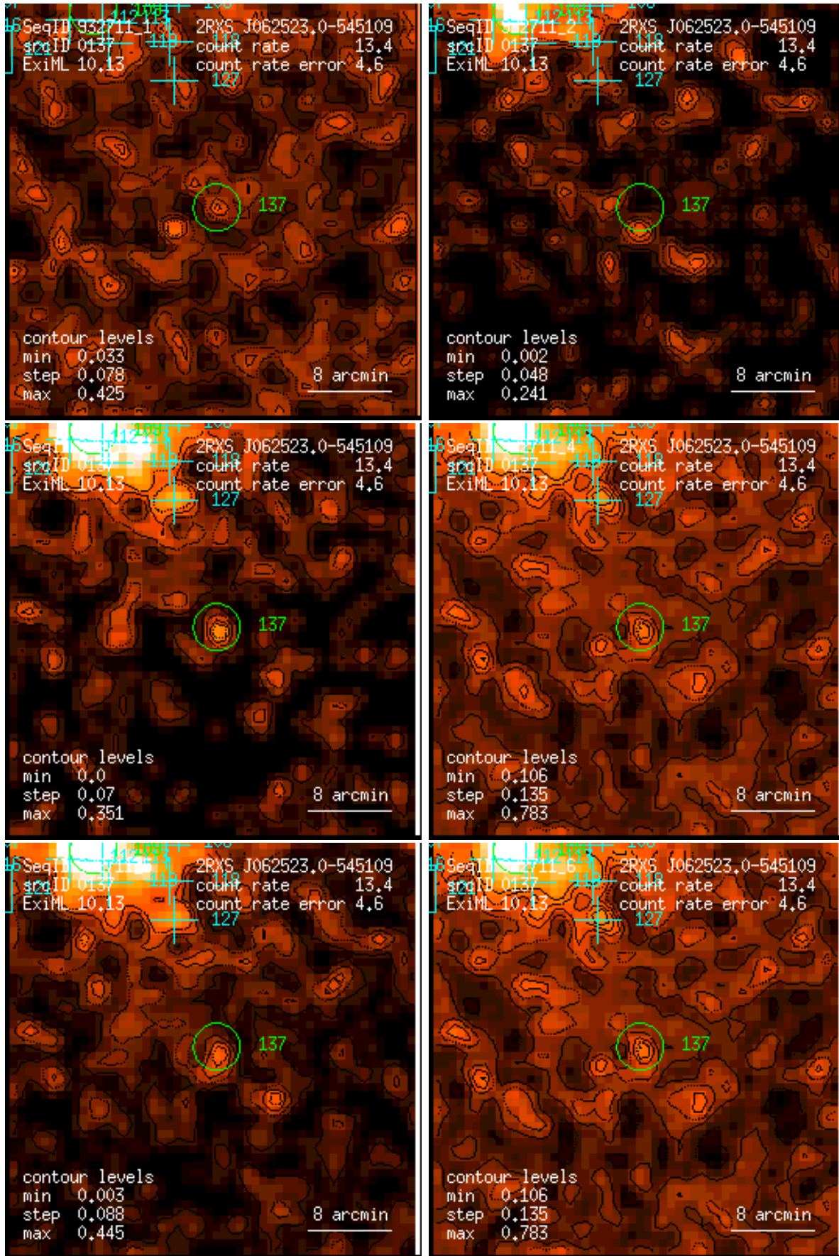
Figure 137: RASS 932711: detection 0137: band rate images, Gaussian filter: (1) PSPC channels 11 – 41, (2) 52 – 90, (3) 91 – 201, (4) 11 – 235, (5) 52 – 201, (6) 11 – 201. Broad band rates in counts/ks. Band rate contour levels in counts/ks/arcmin 2 .
