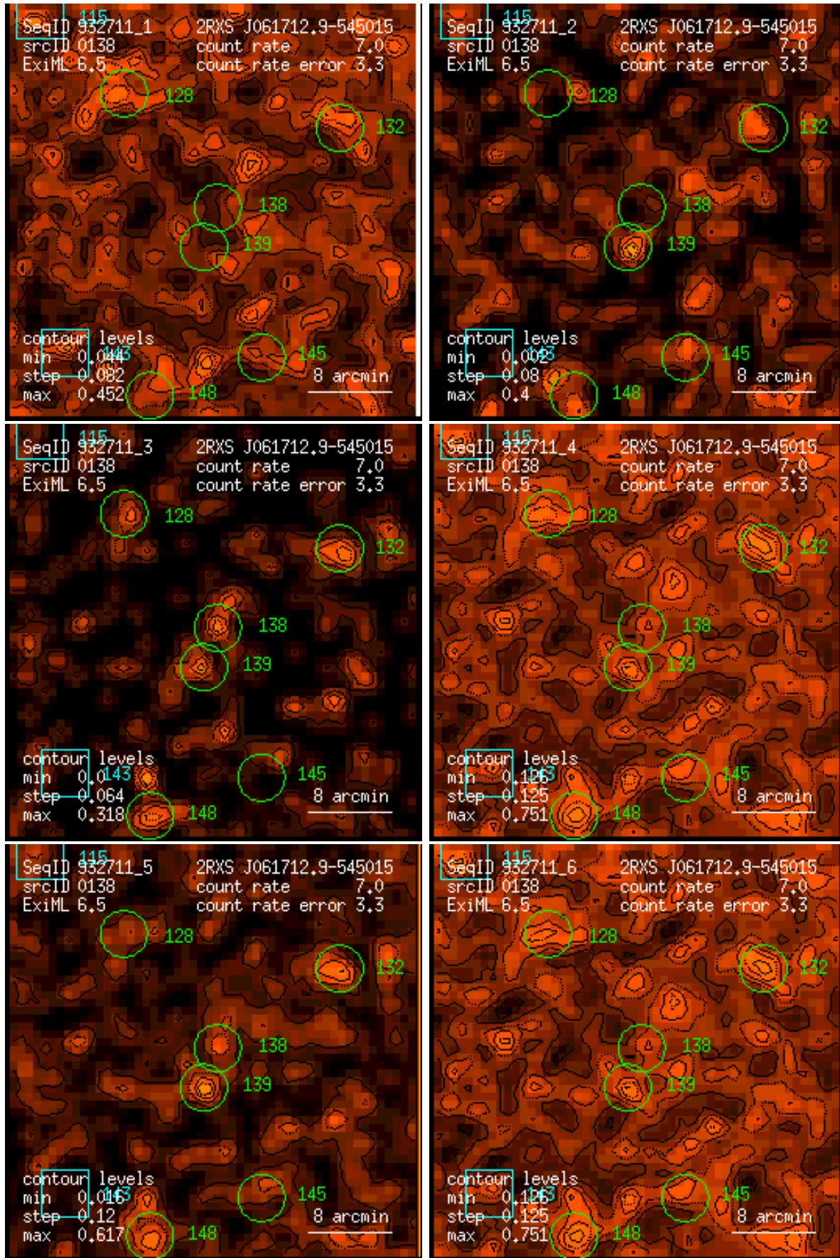
Figure 138: RASS 932711: detection 0138: band rate images, Gaussian filter: (1) PSPC channels 11 – 41, (2) 52 – 90, (3) 91 – 201, (4) 11 – 235, (5) 52 – 201, (6) 11 – 201. Broad band rates in counts/ks. Band rate contour levels in counts/ks/arcmin 2 .
