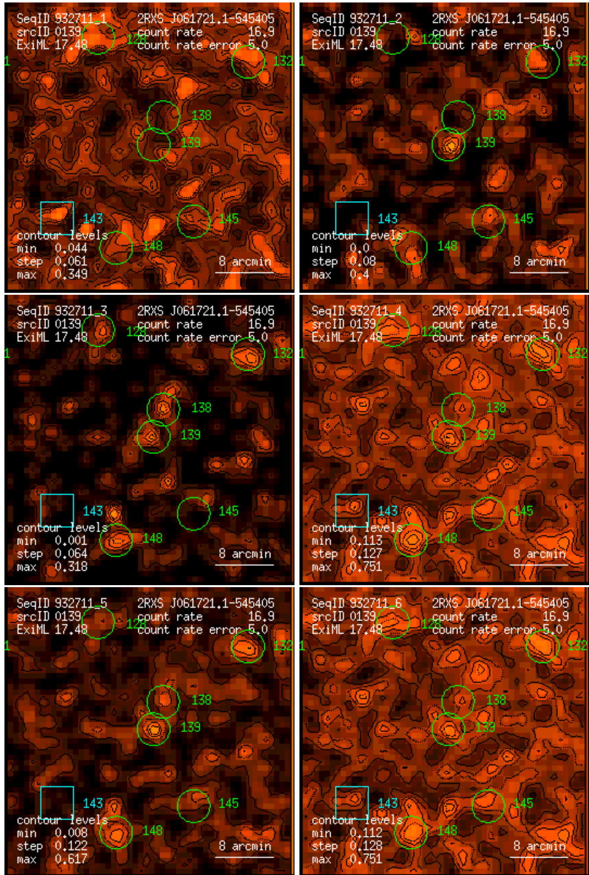
Figure 139: RASS 932711: detection 0139: band rate images, Gaussian filter: (1) PSPC channels 11 – 41, (2) 52 – 90, (3) 91 – 201, (4) 11 – 235, (5) 52 – 201, (6) 11 – 201. Broad band rates in counts/ks. Band rate contour levels in counts/ks/arcmin 2 .
