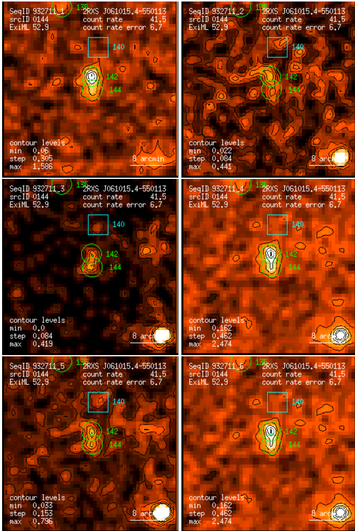
Figure 144: RASS 932711: detection 0144: band rate images, Gaussian filter: (1) PSPC channels 11 – 41, (2) 52 – 90, (3) 91 – 201, (4) 11 – 235, (5) 52 – 201, (6) 11 – 201. Broad band rates in counts/ks. Band rate contour levels in counts/ks/arcmin 2 .
