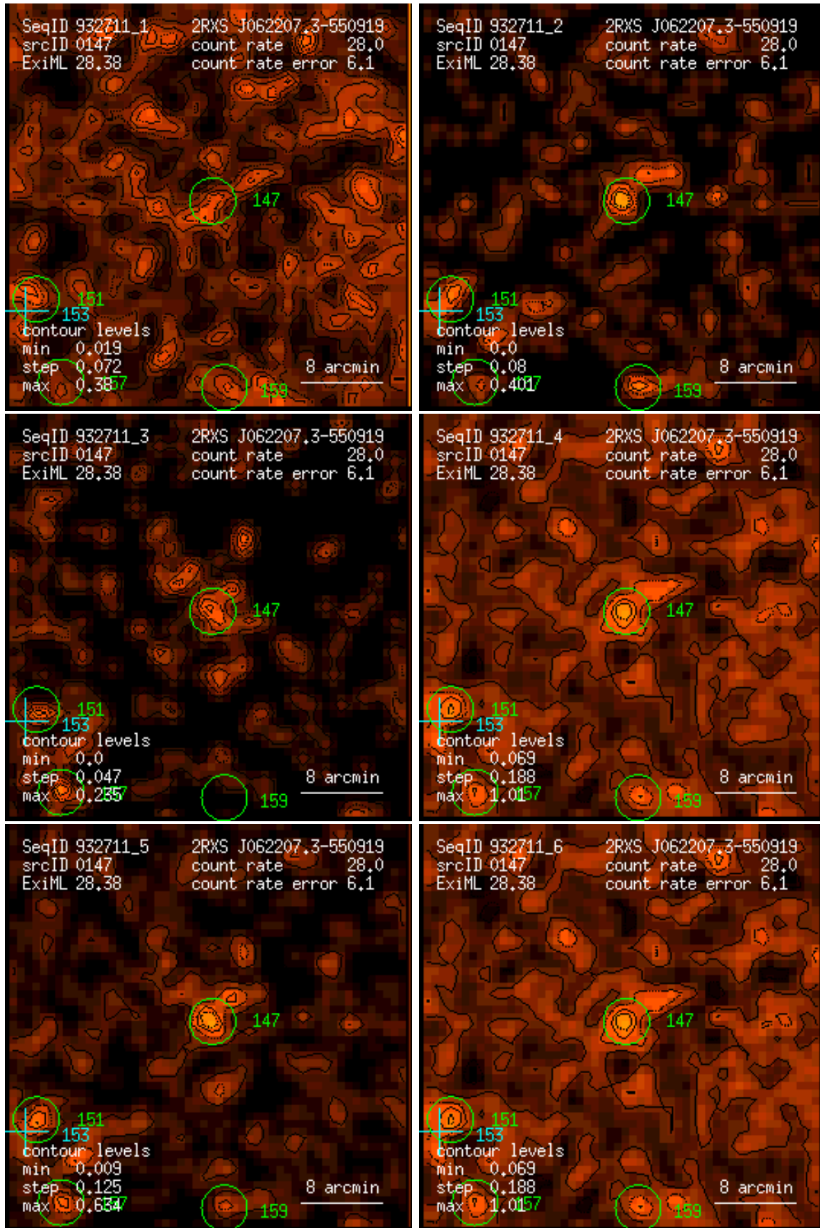
Figure 147: RASS 932711: detection 0147: band rate images, Gaussian filter: (1) PSPC channels 11 – 41, (2) 52 – 90, (3) 91 – 201, (4) 11 – 235, (5) 52 – 201, (6) 11 – 201. Broad band rates in counts/ks. Band rate contour levels in counts/ks/arcmin 2 .
