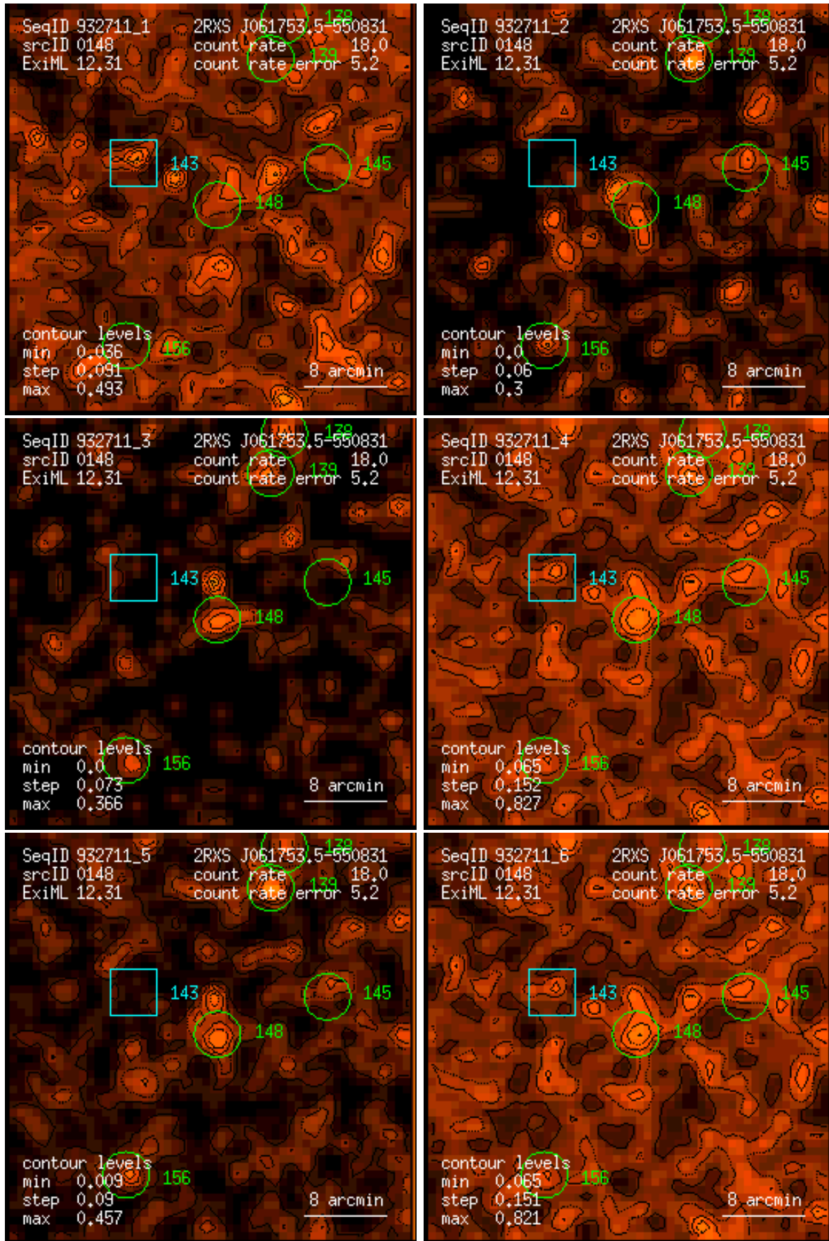
Figure 148: RASS 932711: detection 0148: band rate images, Gaussian filter: (1) PSPC channels 11 – 41, (2) 52 – 90, (3) 91 – 201, (4) 11 – 235, (5) 52 – 201, (6) 11 – 201. Broad band rates in counts/ks. Band rate contour levels in counts/ks/arcmin 2 .
