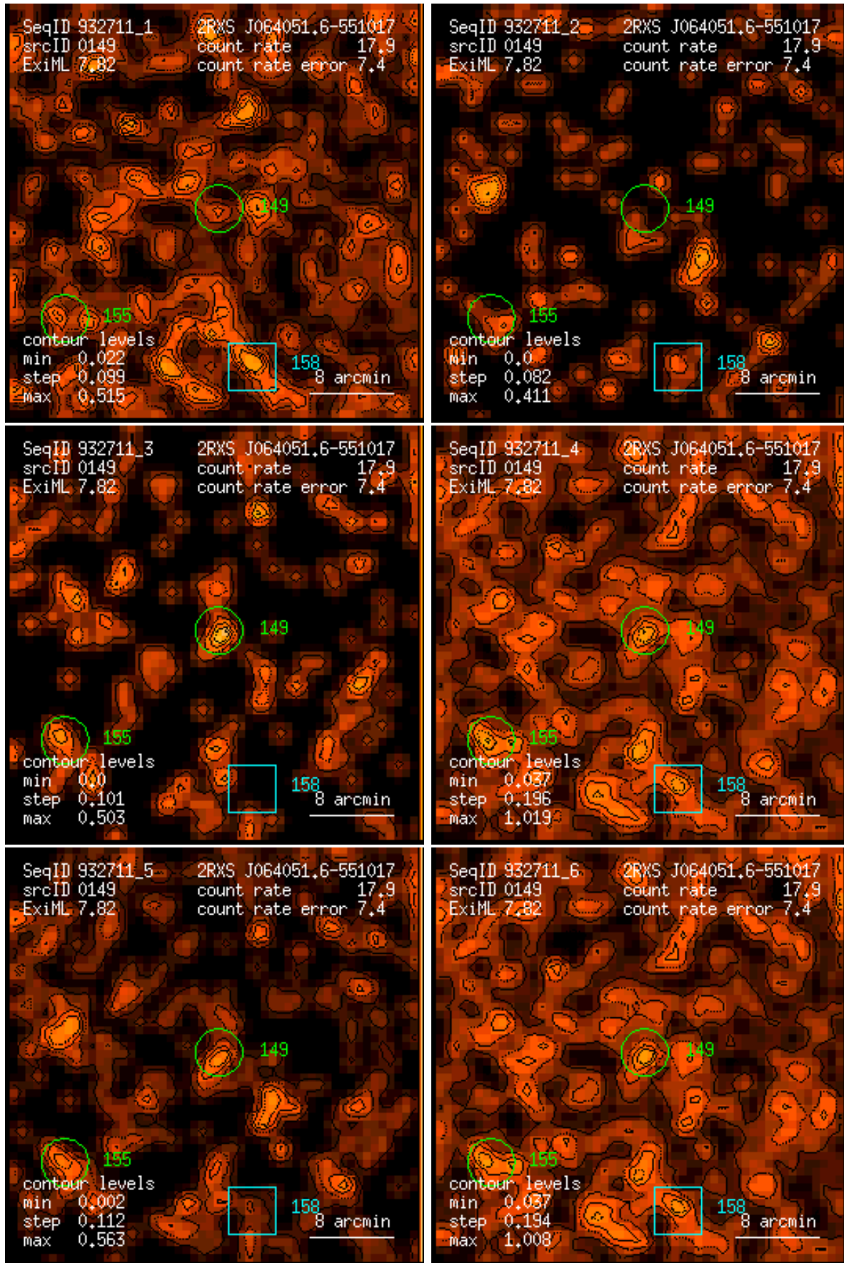
Figure 149: RASS 932711: detection 0149: band rate images, Gaussian filter: (1) PSPC channels 11 – 41, (2) 52 – 90, (3) 91 – 201, (4) 11 – 235, (5) 52 – 201, (6) 11 – 201. Broad band rates in counts/ks. Band rate contour levels in counts/ks/arcmin 2 .
