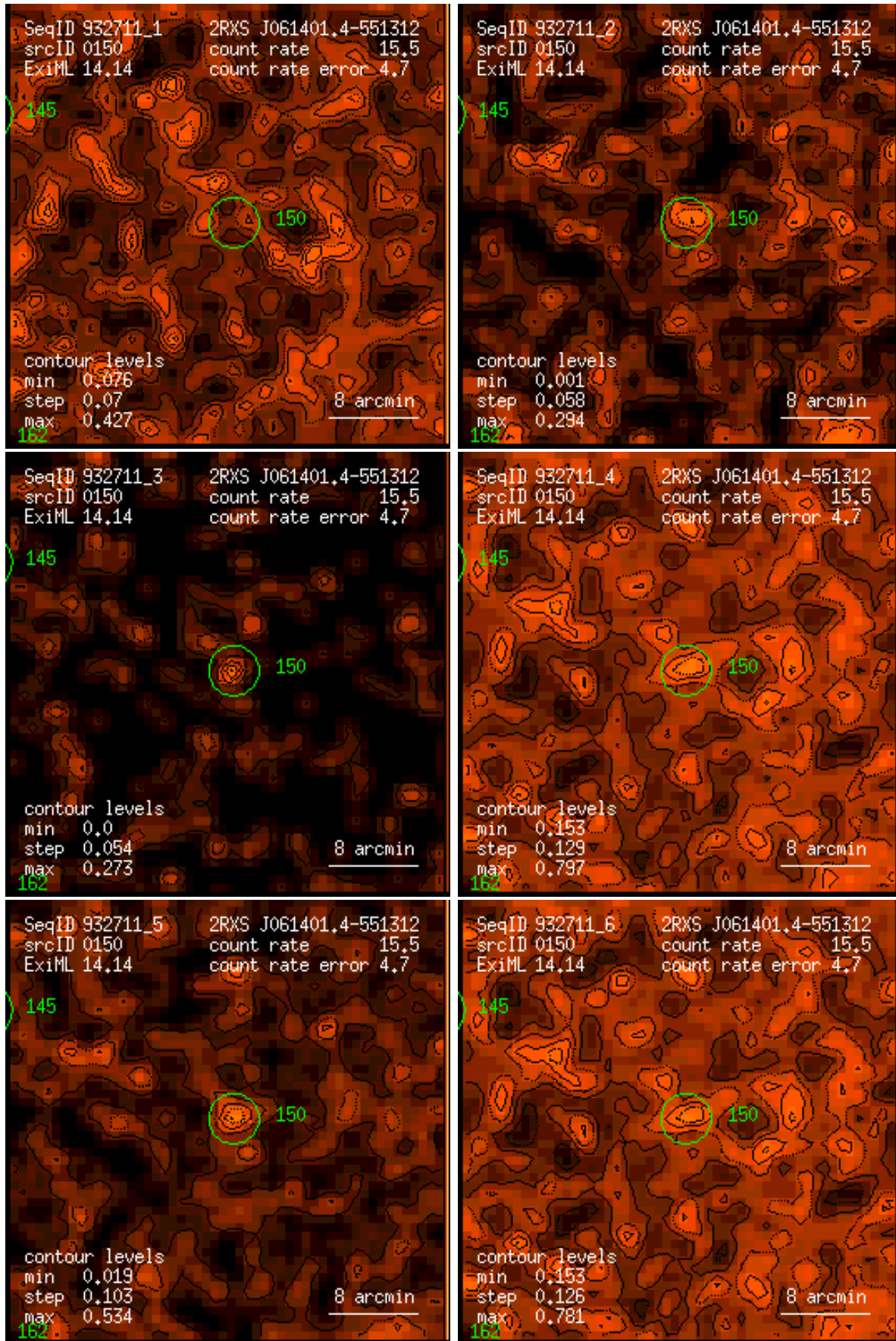
Figure 150: RASS 932711: detection 0150: band rate images, Gaussian filter: (1) PSPC channels 11 – 41, (2) 52 – 90, (3) 91 – 201, (4) 11 – 235, (5) 52 – 201, (6) 11 – 201. Broad band rates in counts/ks. Band rate contour levels in counts/ks/arcmin 2 .
