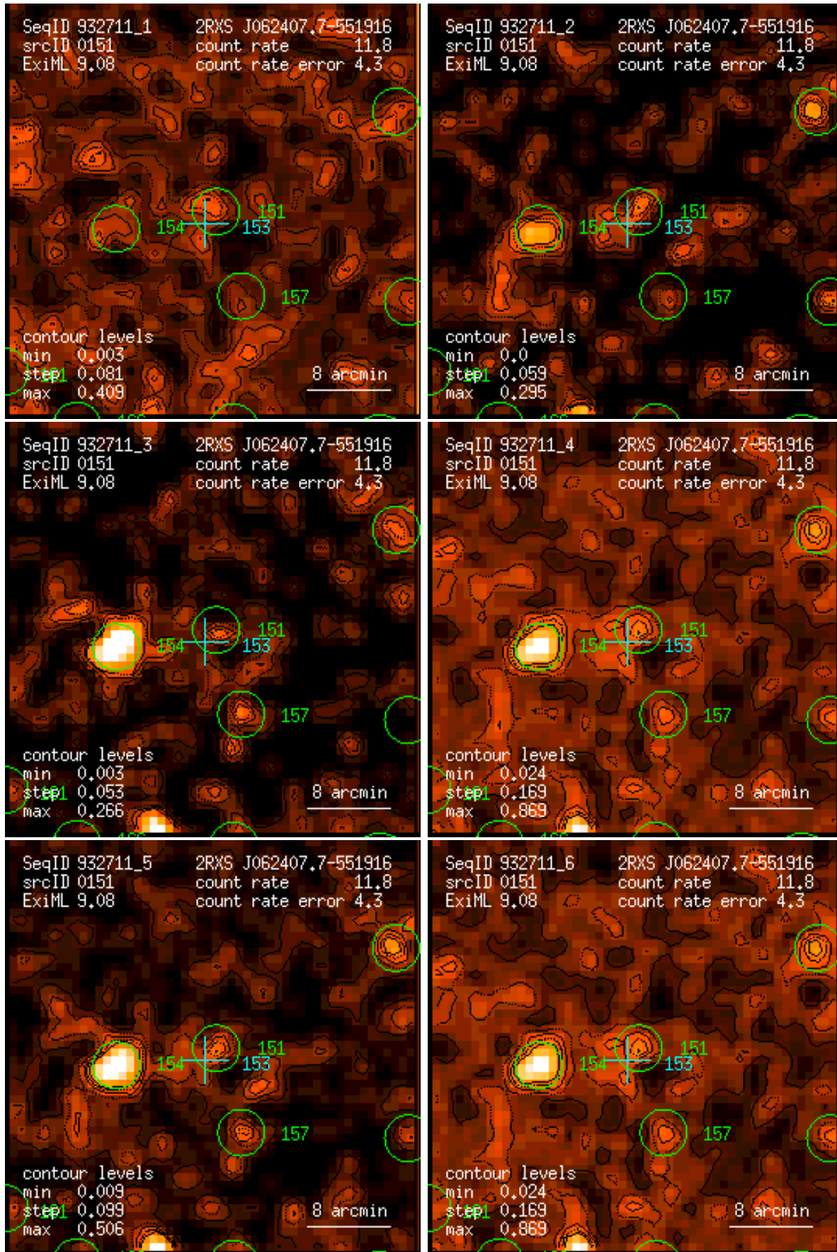
Figure 151: RASS 932711: detection 0151: band rate images, Gaussian filter: (1) PSPC channels 11 – 41, (2) 52 – 90, (3) 91 – 201, (4) 11 – 235, (5) 52 – 201, (6) 11 – 201. Broad band rates in counts/ks. Band rate contour levels in counts/ks/arcmin 2 .
