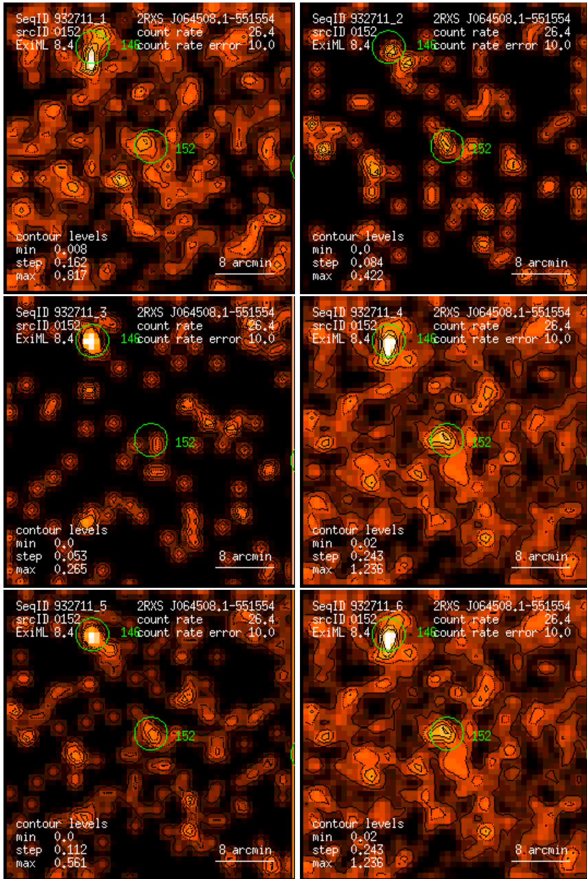
Figure 152: RASS 932711: detection 0152: band rate images, Gaussian filter: (1) PSPC channels 11 – 41, (2) 52 – 90, (3) 91 – 201, (4) 11 – 235, (5) 52 – 201, (6) 11 – 201. Broad band rates in counts/ks. Band rate contour levels in counts/ks/arcmin 2 .
