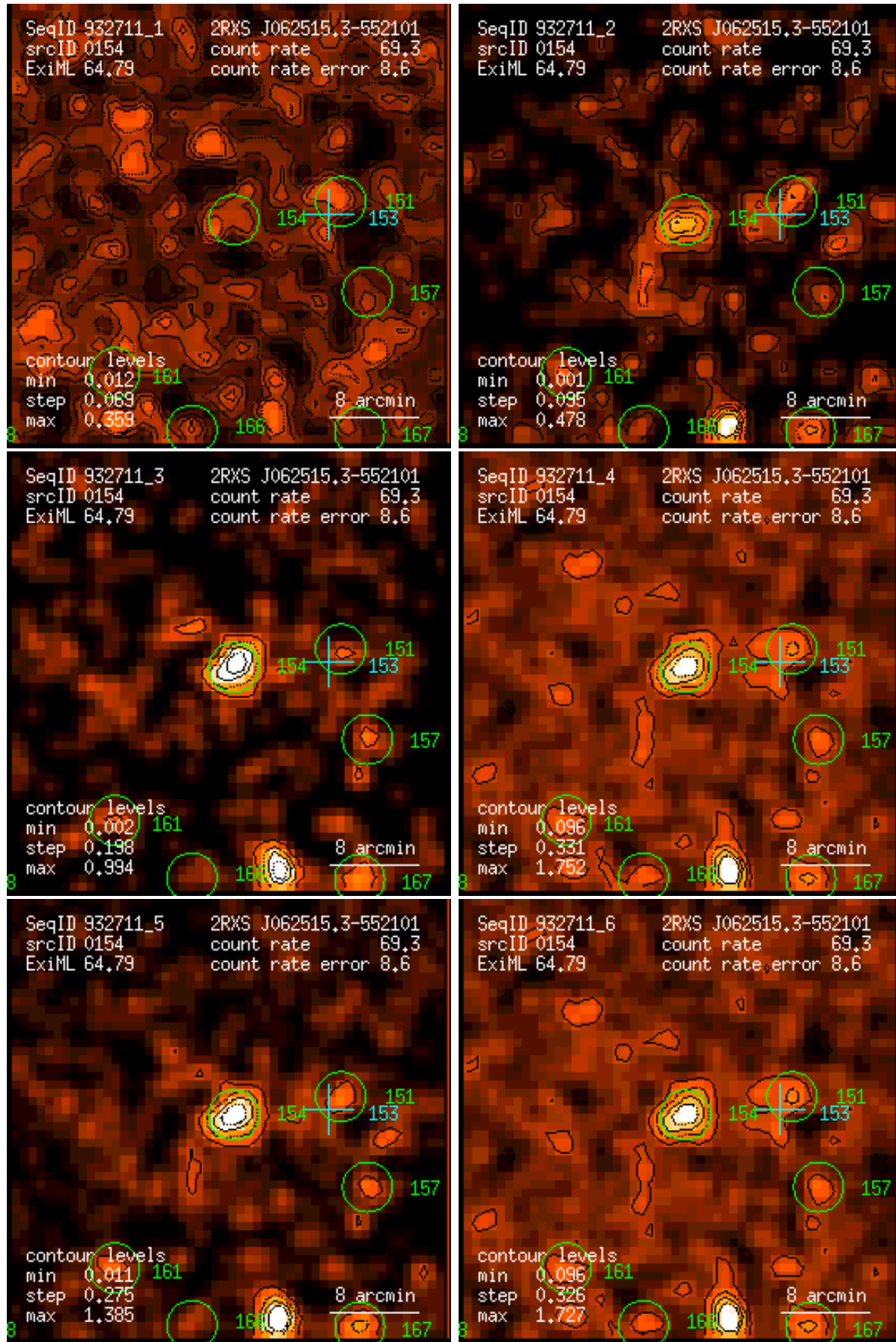
Figure 154: RASS 932711: detection 0154: band rate images, Gaussian filter: (1) PSPC channels 11 – 41, (2) 52 – 90, (3) 91 – 201, (4) 11 – 235, (5) 52 – 201, (6) 11 – 201. Broad band rates in counts/ks. Band rate contour levels in counts/ks/arcmin 2 .
