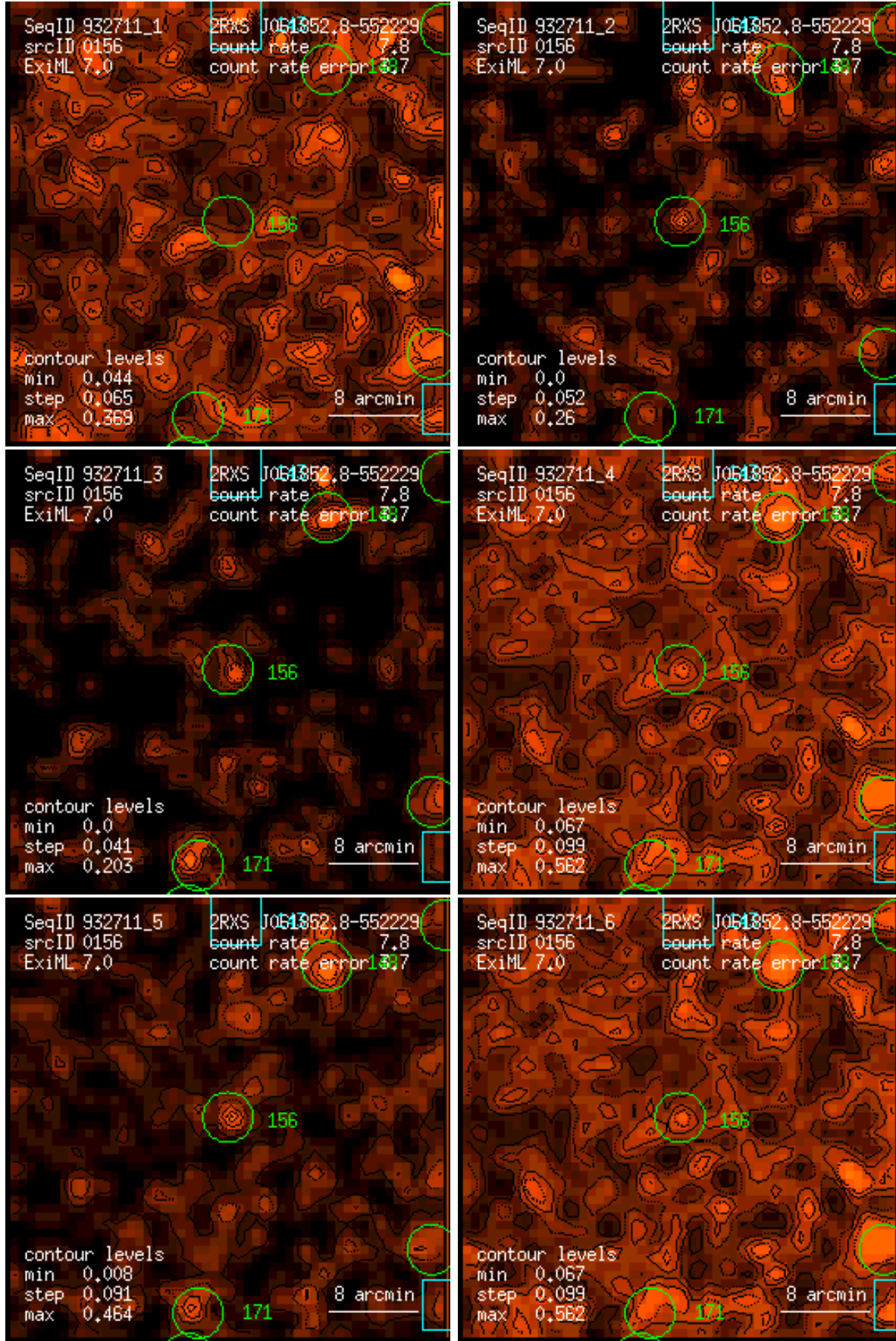
Figure 156: RASS 932711: detection 0156: band rate images, Gaussian filter: (1) PSPPC channels 11 – 41, (2) 52 – 90, (3) 91 – 201, (4) 11 – 235, (5) 52 – 201, (6) 11 – 201. Broad band rates in counts/ks. Band rate contour levels in counts/ks/arcmin 2 .
