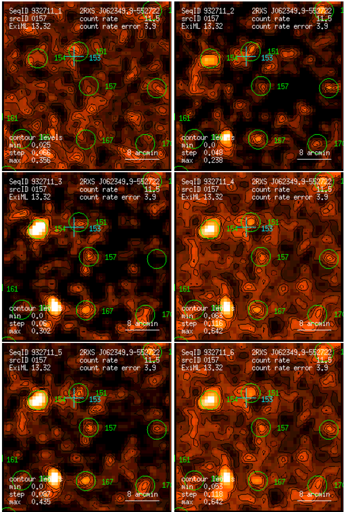
Figure 157: RASS 932711: detection 0157: band rate images, Gaussian filter: (1) PSPC channels 11 – 41, (2) 52 – 90, (3) 91 – 201, (4) 11 – 235, (5) 52 – 201, (6) 11 – 201. Broad band rates in counts/ks. Band rate contour levels in counts/ks/arcmin 2 .
