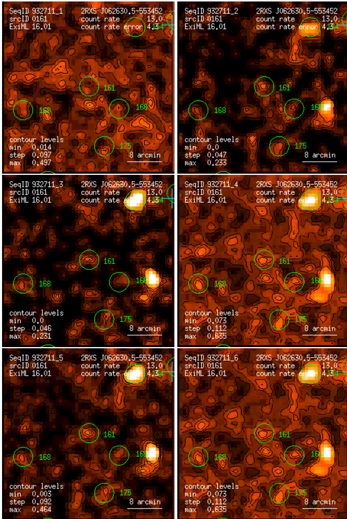
Figure 161: RASS 932711: detection 0161: band rate images, Gaussian filter: (1) PSPC channels 11 – 41, (2) 52 – 90, (3) 91 – 201, (4) 11 – 235, (5) 52 – 201, (6) 11 – 201. Broad band rates in counts/ks. Band rate contour levels in counts/ks/arcmin 2 .
