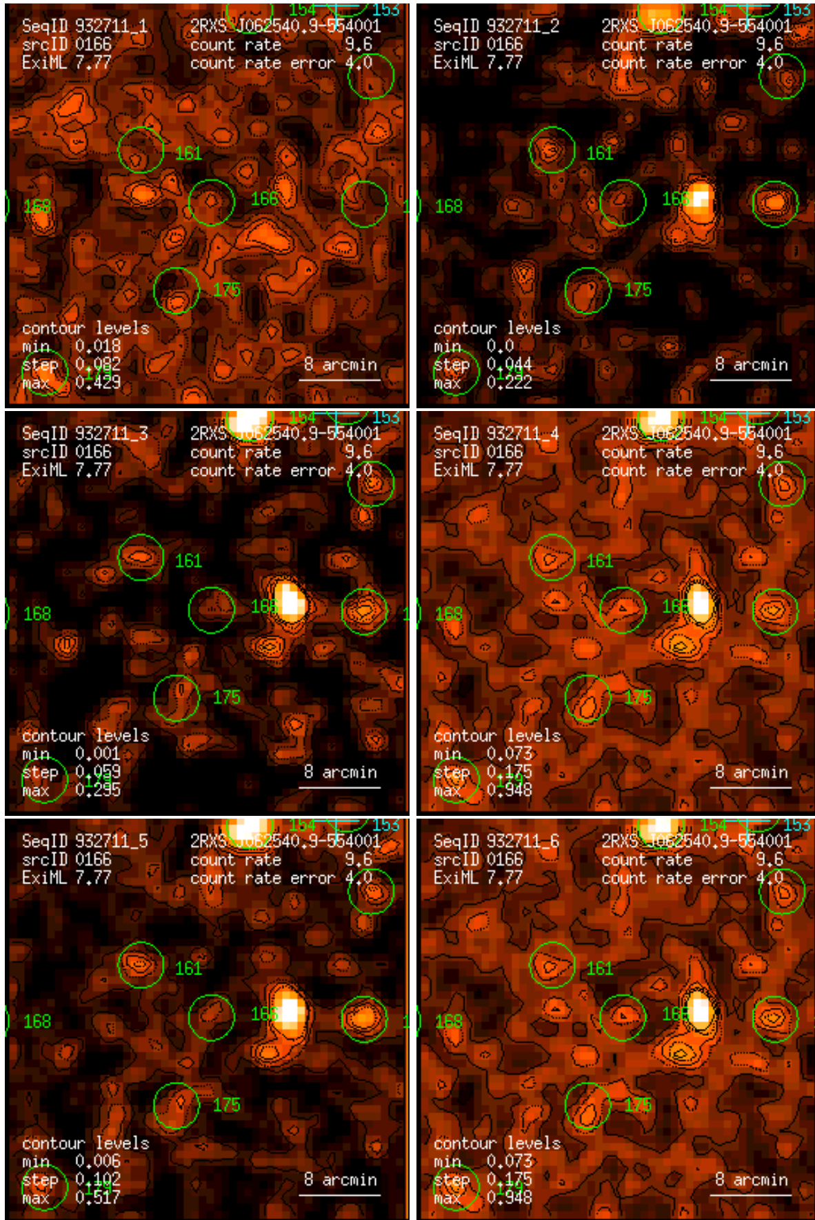
Figure 166: RASS 932711: detection 0166: band rate images, Gaussian filter: (1) PSPC channels 11 – 41, (2) 52 – 90, (3) 91 – 201, (4) 11 – 235, (5) 52 – 201, (6) 11 – 201. Broad band rates in counts/ks. Band rate contour levels in counts/ks/arcmin 2 .
