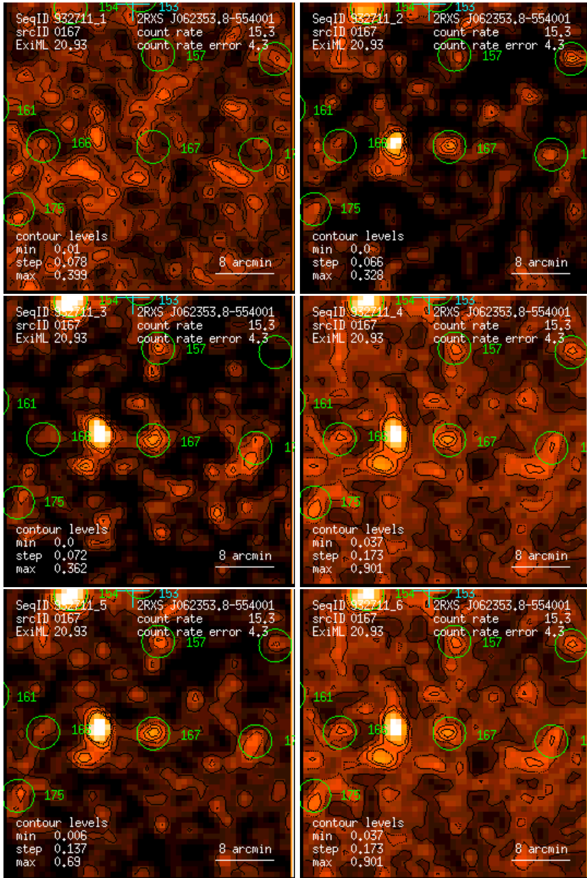
Figure 167: RASS 932711: detection 0167: band rate images, Gaussian filter: (1) PSPC channels 11 – 41, (2) 52 – 90, (3) 91 – 201, (4) 11 – 235, (5) 52 – 201, (6) 11 – 201. Broad band rates in counts/ks. Band rate contour levels in counts/ks/arcmin 2 .
