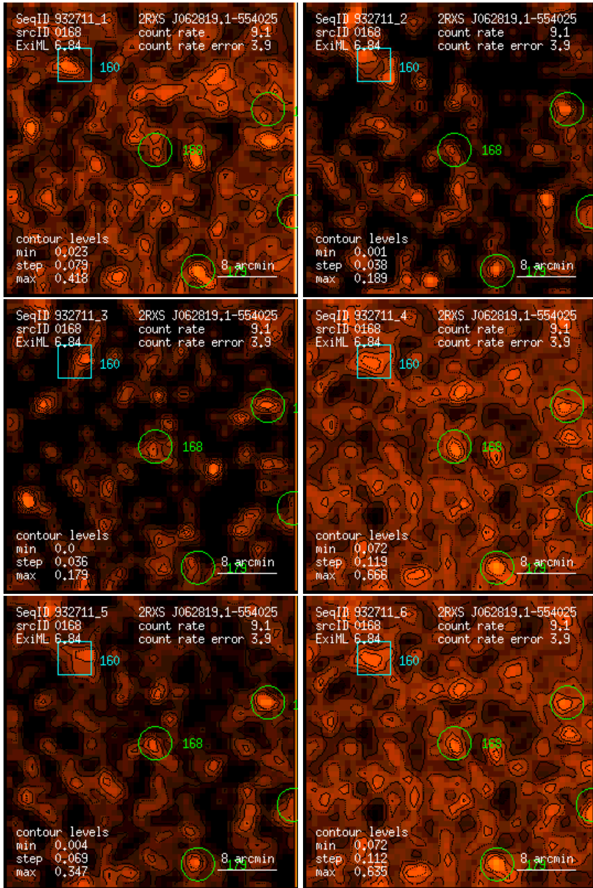
Figure 168: RASS 932711: detection 0168: band rate images, Gaussian filter: (1) PSPC channels 11 – 41, (2) 52 – 90, (3) 91 – 201, (4) 11 – 235, (5) 52 – 201, (6) 11 – 201. Broad band rates in counts/ks. Band rate contour levels in counts/ks/arcmin 2 .
