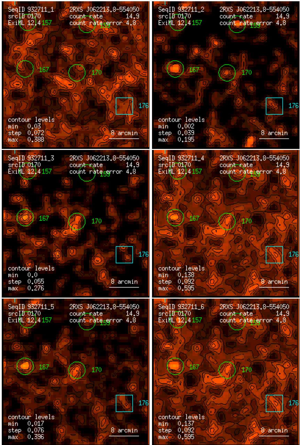
Figure 170: RASS 932711: detection 0170: band rate images, Gaussian filter: (1) PSPC channels 11 – 41, (2) 52 – 90, (3) 91 – 201, (4) 11 – 235, (5) 52 – 201, (6) 11 – 201. Broad band rates in counts/ks. Band rate contour levels in counts/ks/arcmin 2 .
