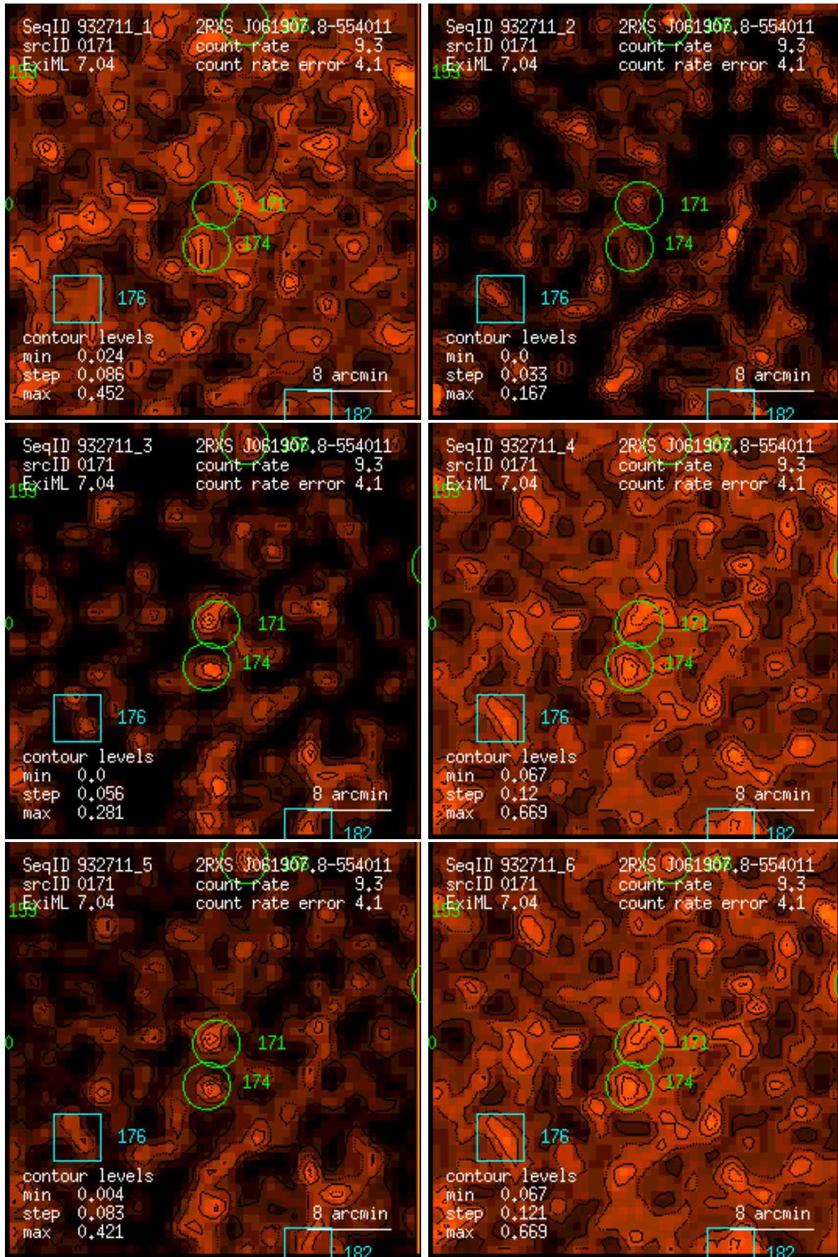
Figure 171: RASS 932711: detection 0171: band rate images, Gaussian filter: (1) PSPC channels 11 – 41, (2) 52 – 90, (3) 91 – 201, (4) 11 – 235, (5) 52 – 201, (6) 11 – 201. Broad band rates in counts/ks. Band rate contour levels in counts/ks/arcmin 2 .
