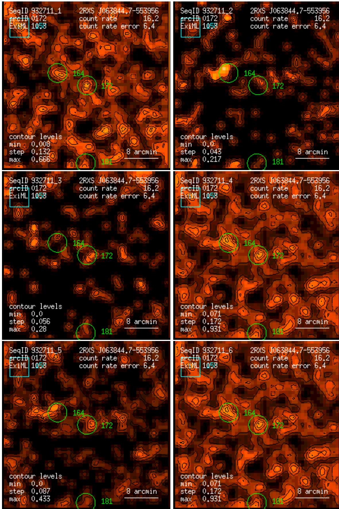
Figure 172: RASS 932711: detection 0172: band rate images, Gaussian filter: (1) PSPC channels 11 – 41, (2) 52 – 90, (3) 91 – 201, (4) 11 – 235, (5) 52 – 201, (6) 11 – 201. Broad band rates in counts/ks. Band rate contour levels in counts/ks/arcmin 2 .
