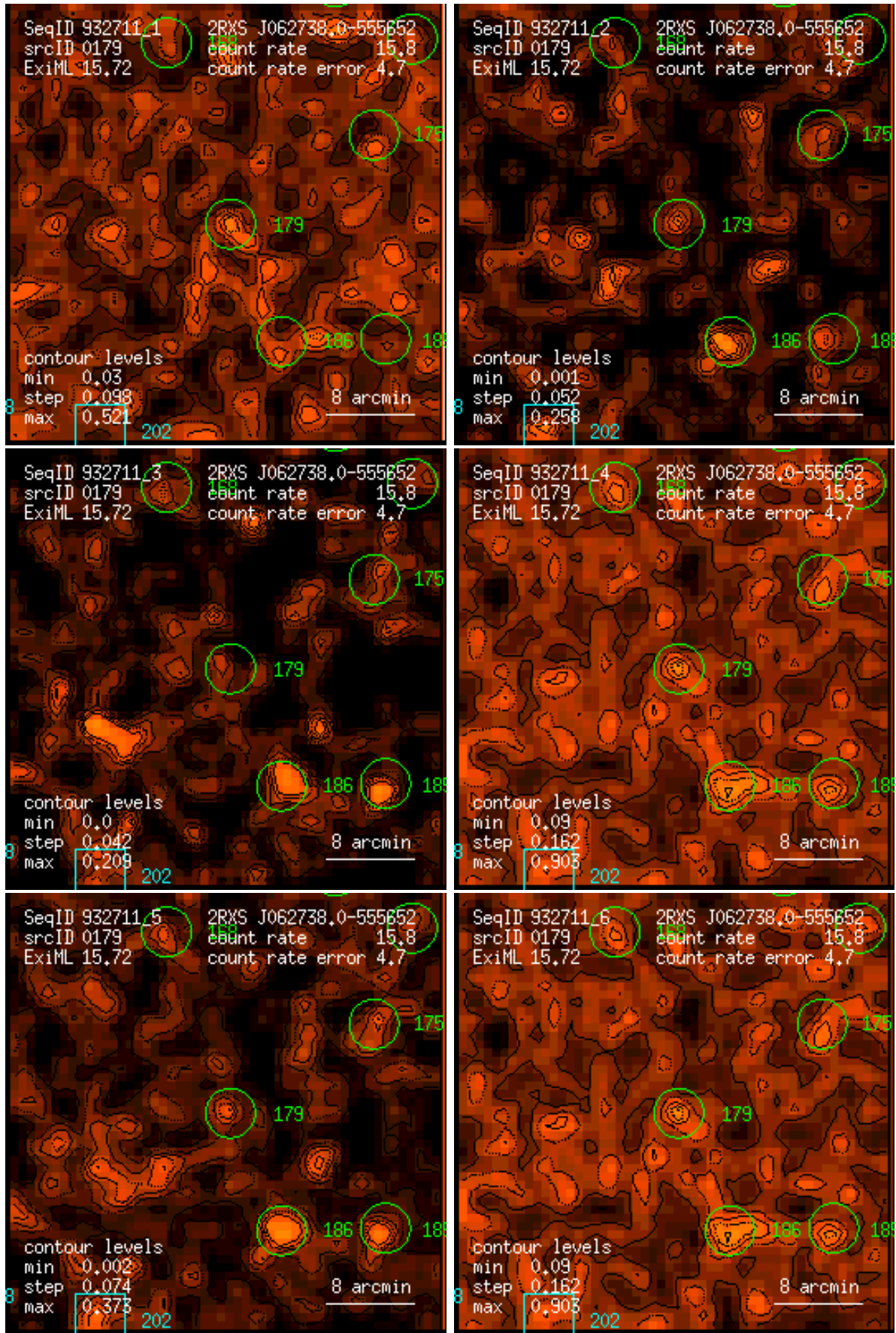
Figure 179: RASS 932711: detection 0179: band rate images, Gaussian filter: (1) PSPC channels 11 – 41, (2) 52 – 90, (3) 91 – 201, (4) 11 – 235, (5) 52 – 201, (6) 11 – 201. Broad band rates in counts/ks. Band rate contour levels in counts/ks/arcmin 2 .
