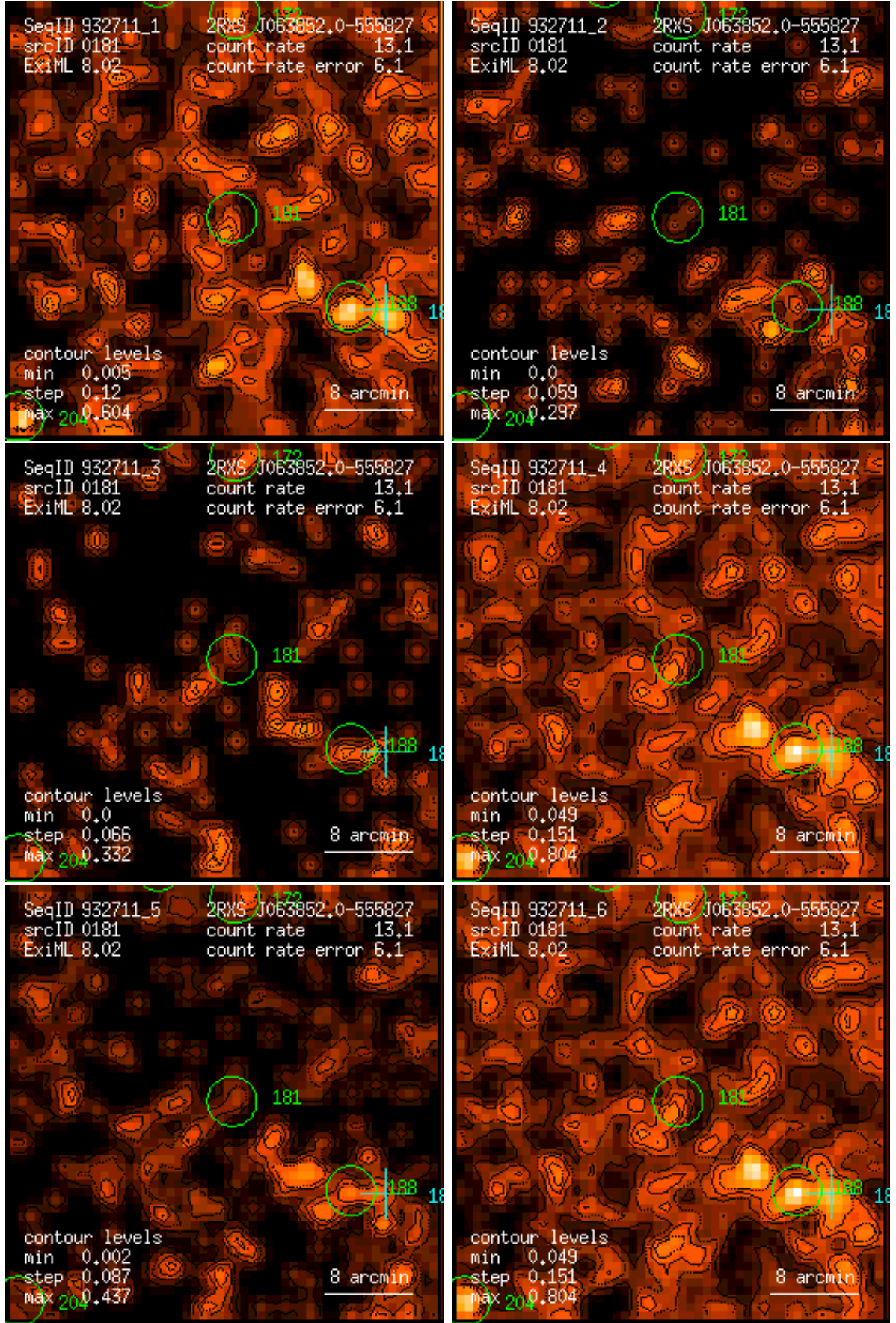
Figure 181: RASS 932711: detection 0181: band rate images, Gaussian filter: (1) PSPC channels 11 – 41, (2) 52 – 90, (3) 91 – 201, (4) 11 – 235, (5) 52 – 201, (6) 11 – 201. Broad band rates in counts/ks. Band rate contour levels in counts/ks/arcmin 2 .
