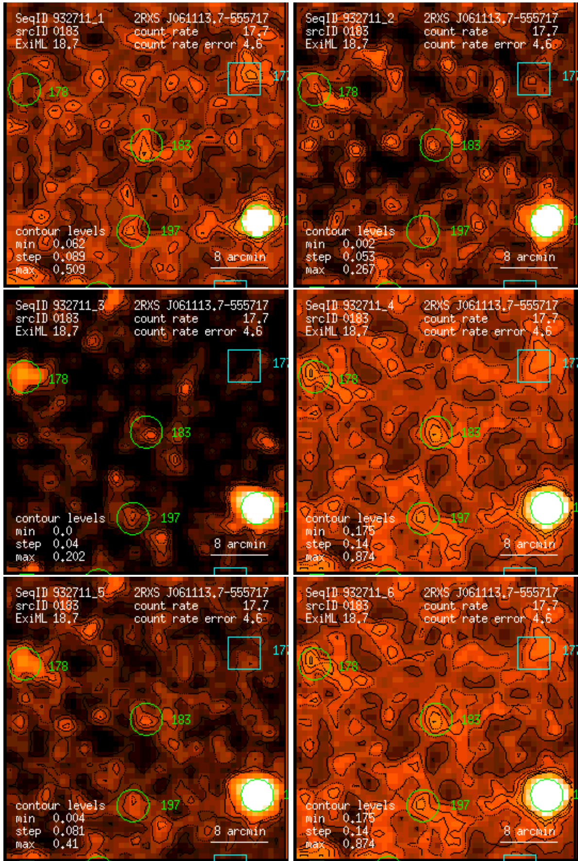
Figure 183: RASS 932711: detection 0183: band rate images, Gaussian filter: (1) PSPC channels 11 – 41, (2) 52 – 90, (3) 91 – 201, (4) 11 – 235, (5) 52 – 201, (6) 11 – 201. Broad band rates in counts/ks. Band rate contour levels in counts/ks/arcmin 2 .
