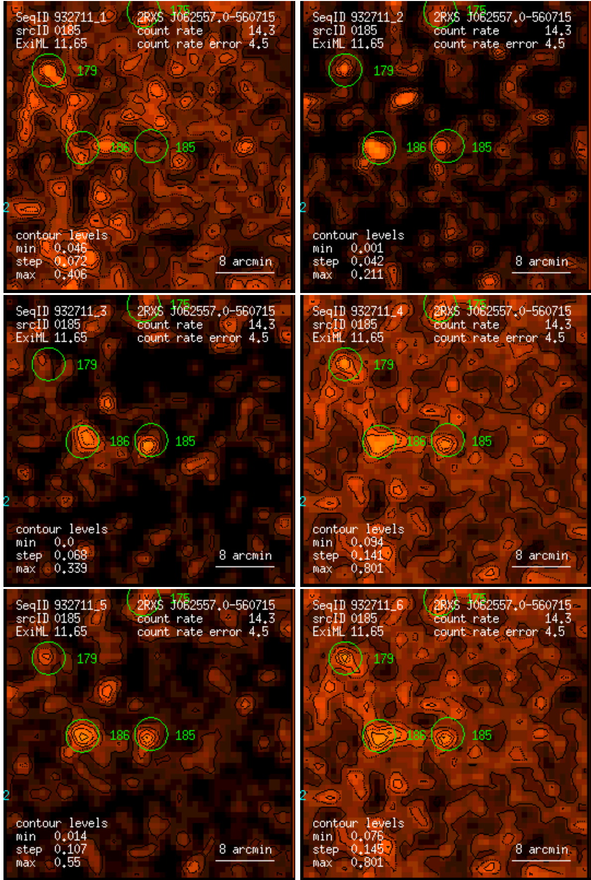
Figure 185: RASS 932711: detection 0185: band rate images, Gaussian filter: (1) PSPC channels 11 – 41, (2) 52 – 90, (3) 91 – 201, (4) 11 – 235, (5) 52 – 201, (6) 11 – 201. Broad band rates in counts/ks. Band rate contour levels in counts/ks/arcmin 2 .
