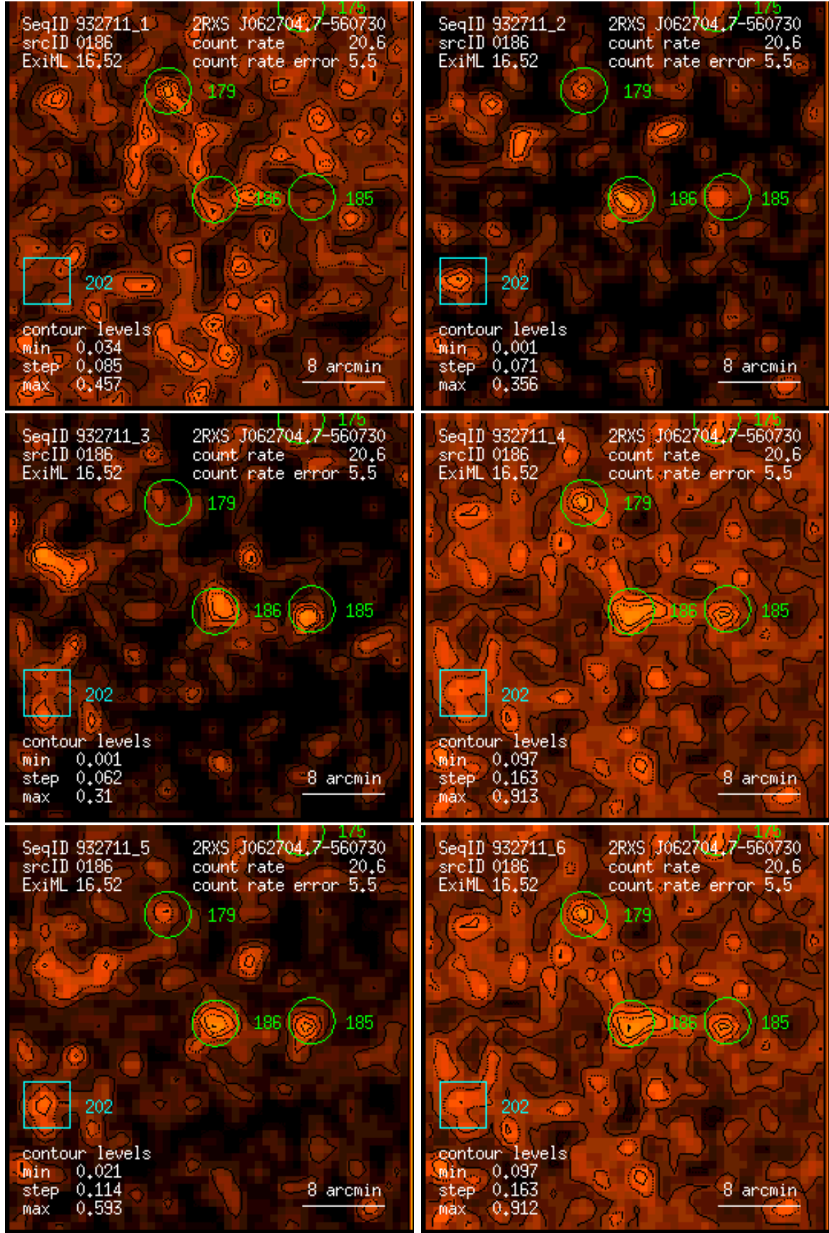
Figure 186: RASS 932711: detection 0186: band rate images, Gaussian filter: (1) PSPC channels 11 – 41, (2) 52 – 90, (3) 91 – 201, (4) 11 – 235, (5) 52 – 201, (6) 11 – 201. Broad band rates in counts/ks. Band rate contour levels in counts/ks/arcmin 2 .
