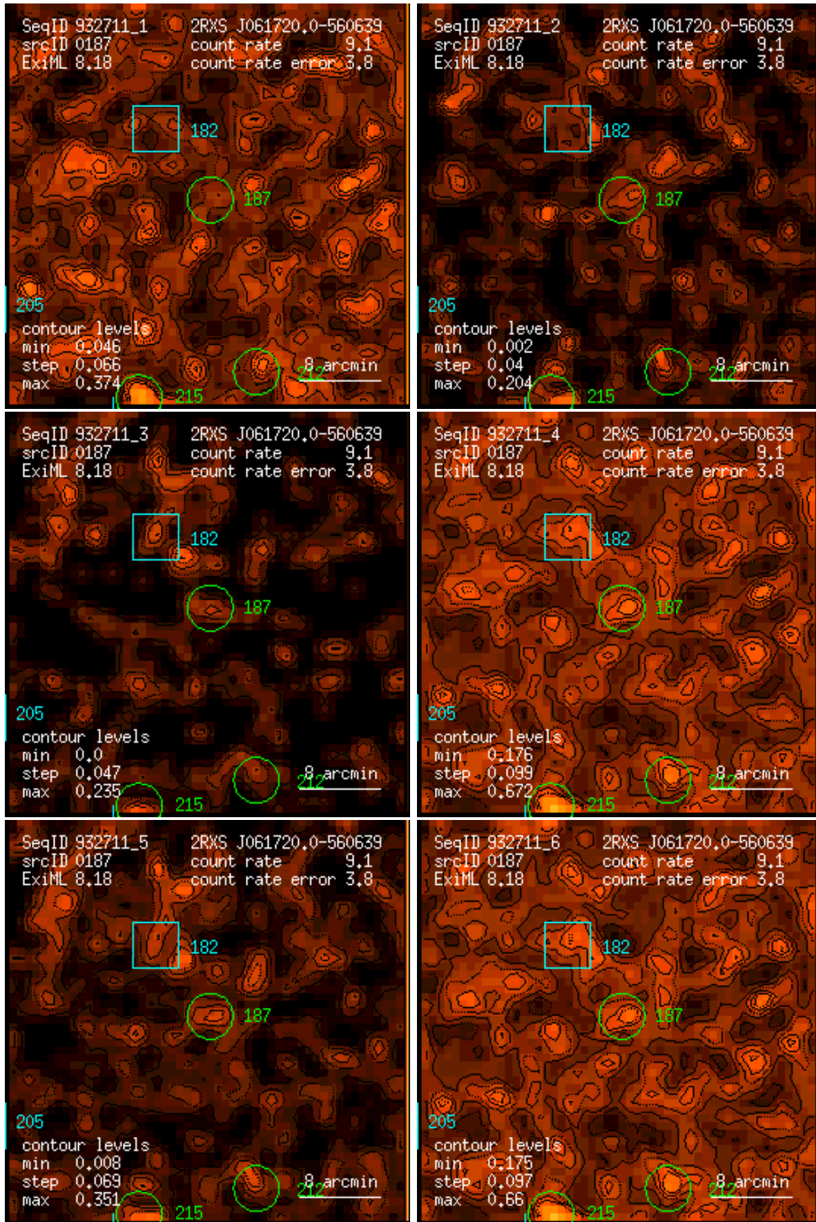
Figure 187: RASS 932711: detection 0187: band rate images, Gaussian filter: (1) PSPC channels 11 – 41, (2) 52 – 90, (3) 91 – 201, (4) 11 – 235, (5) 52 – 201, (6) 11 – 201. Broad band rates in counts/ks. Band rate contour levels in counts/ks/arcmin 2 .
