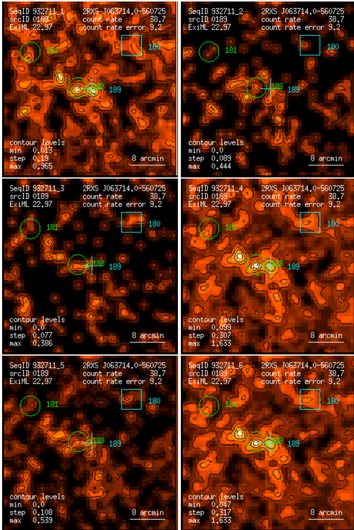
Figure 189: RASS 932711: detection 0189: band rate images, Gaussian filter: (1) PSPC channels 11 – 41, (2) 52 – 90, (3) 91 – 201, (4) 11 – 235, (5) 52 – 201, (6) 11 – 201. Broad band rates in counts/ks. Band rate contour levels in counts/ks/arcmin 2 .
