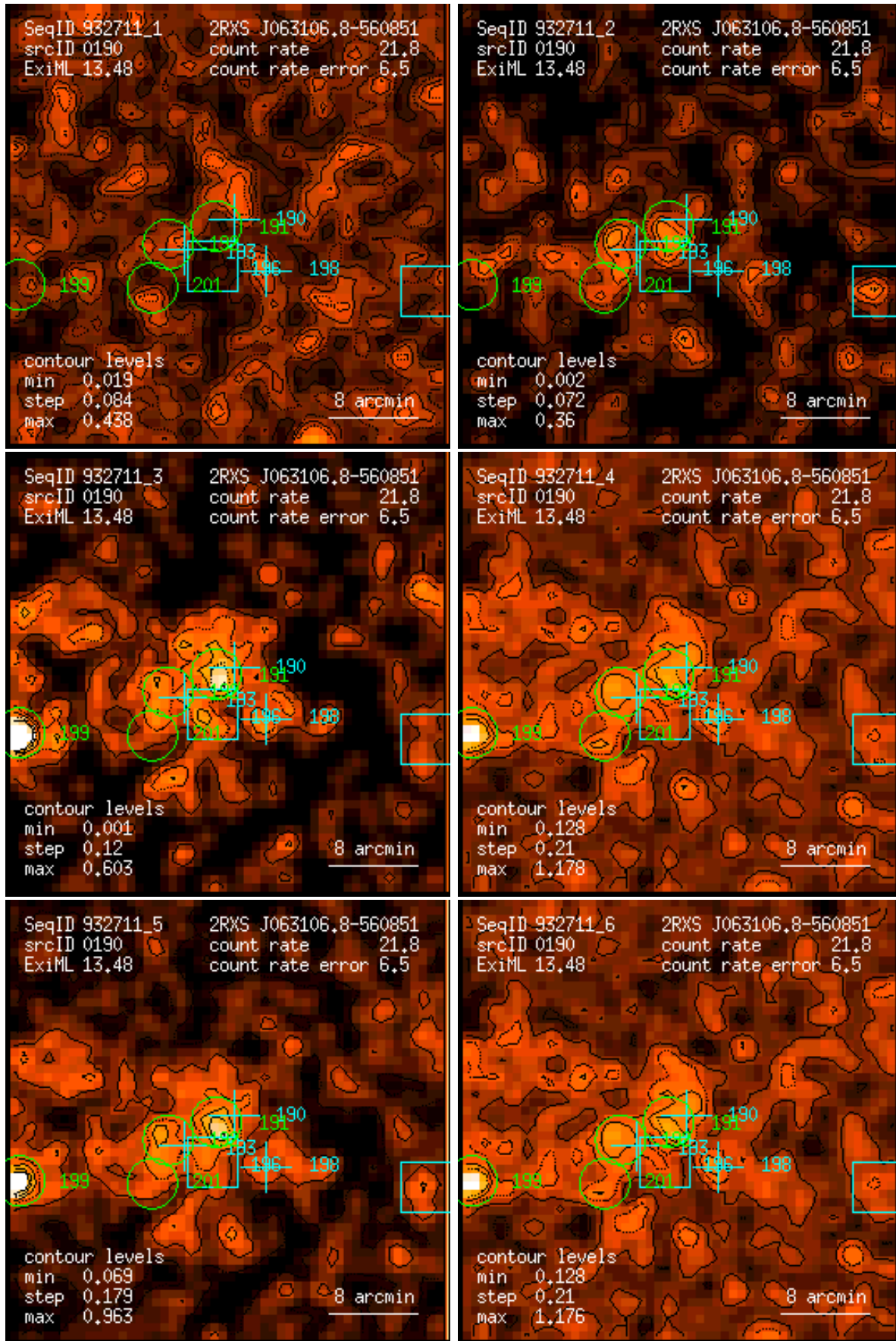
Figure 190: RASS 932711: detection 0190: band rate images, Gaussian filter: (1) PSPC channels 11 – 41, (2) 52 – 90, (3) 91 – 201, (4) 11 – 235, (5) 52 – 201, (6) 11 – 201. Broad band rates in counts/ks. Band rate contour levels in counts/ks/arcmin 2 .
