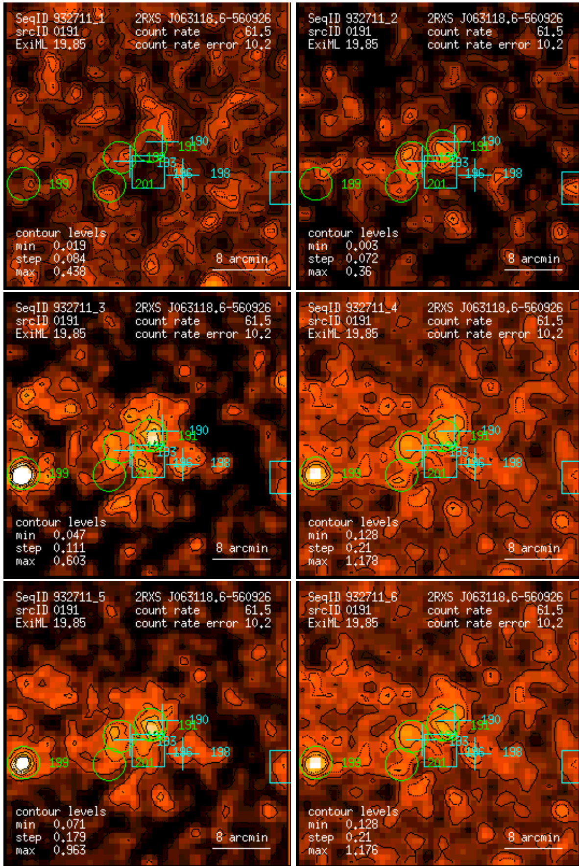
Figure 191: RASS 932711: detection 0191: band rate images, Gaussian filter: (1) PSPC channels 11 – 41, (2) 52 – 90, (3) 91 – 201, (4) 11 – 235, (5) 52 – 201, (6) 11 – 201. Broad band rates in counts/ks. Band rate contour levels in counts/ks/arcmin 2 .
