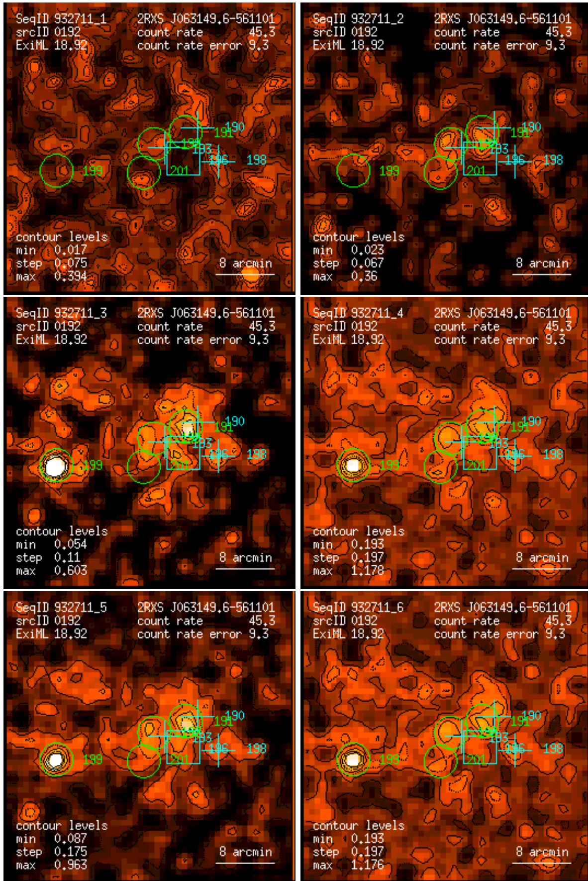
Figure 192: RASS 932711: detection 0192: band rate images, Gaussian filter: (1) PSPC channels 11 – 41, (2) 52 – 90, (3) 91 – 201, (4) 11 – 235, (5) 52 – 201, (6) 11 – 201. Broad band rates in counts/ks. Band rate contour levels in counts/ks/arcmin 2 .
