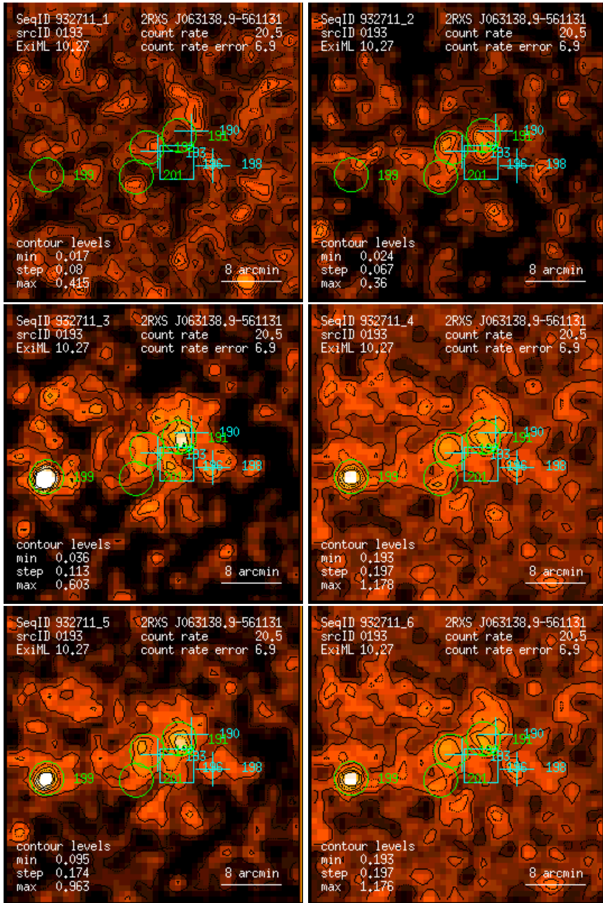
Figure 193: RASS 932711: detection 0193: band rate images, Gaussian filter: (1) PSPC channels 11 – 41, (2) 52 – 90, (3) 91 – 201, (4) 11 – 235, (5) 52 – 201, (6) 11 – 201. Broad band rates in counts/ks. Band rate contour levels in counts/ks/arcmin 2 .
