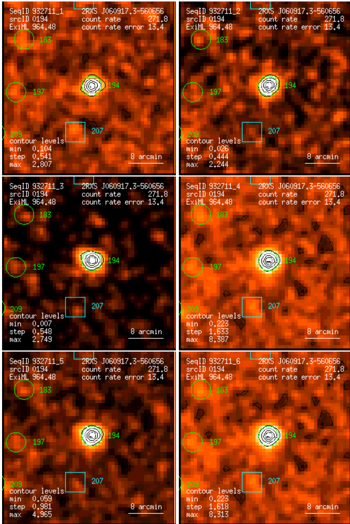
Figure 194: RASS 932711: detection 0194: band rate images, Gaussian filter: (1) PSPC channels 11 – 41, (2) 52 – 90, (3) 91 – 201, (4) 11 – 235, (5) 52 – 201, (6) 11 – 201. Broad band rates in counts/ks. Band rate contour levels in counts/ks/arcmin 2 .
