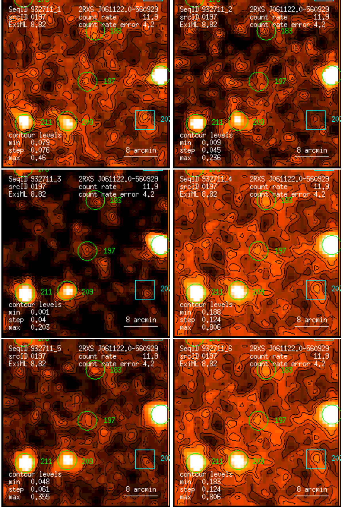
Figure 197: RASS 932711: detection 0197: band rate images, Gaussian filter: (1) PSPC channels 11 – 41, (2) 52 – 90, (3) 91 – 201, (4) 11 – 235, (5) 52 – 201, (6) 11 – 201. Broad band rates in counts/ks. Band rate contour levels in counts/ks/arcmin 2 .
