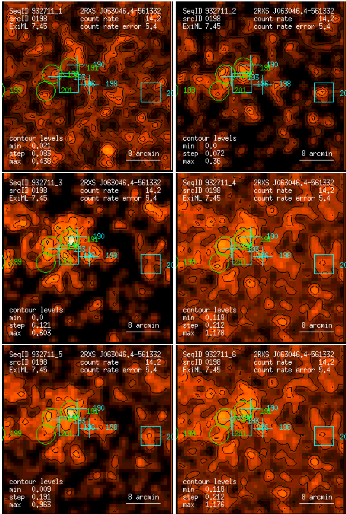
Figure 198: RASS 932711: detection 0198: band rate images, Gaussian filter: (1) PSPC channels 11 – 41, (2) 52 – 90, (3) 91 – 201, (4) 11 – 235, (5) 52 – 201, (6) 11 – 201. Broad band rates in counts/ks. Band rate contour levels in counts/ks/arcmin 2 .
