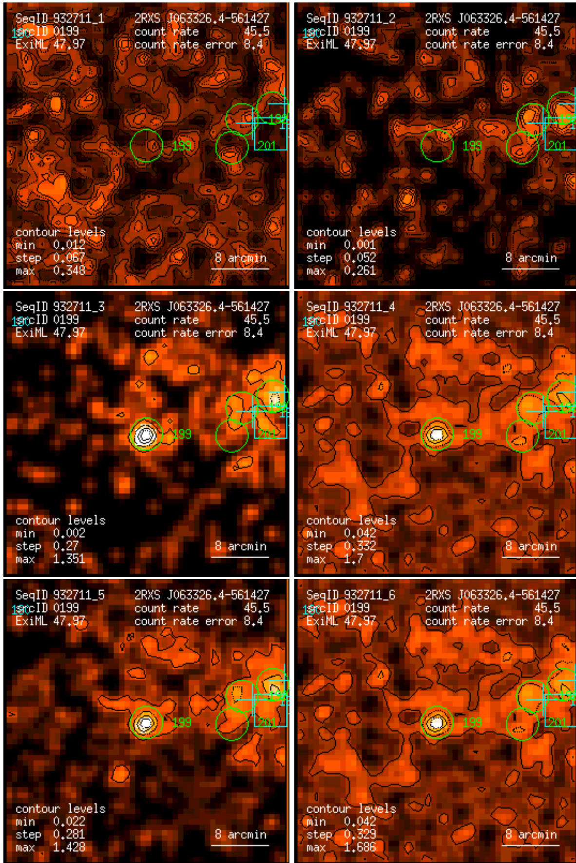
Figure 199: RASS 932711: detection 0199: band rate images, Gaussian filter: (1) PSPC channels 11 – 41, (2) 52 – 90, (3) 91 – 201, (4) 11 – 235, (5) 52 – 201, (6) 11 – 201. Broad band rates in counts/ks. Band rate contour levels in counts/ks/arcmin 2 .
