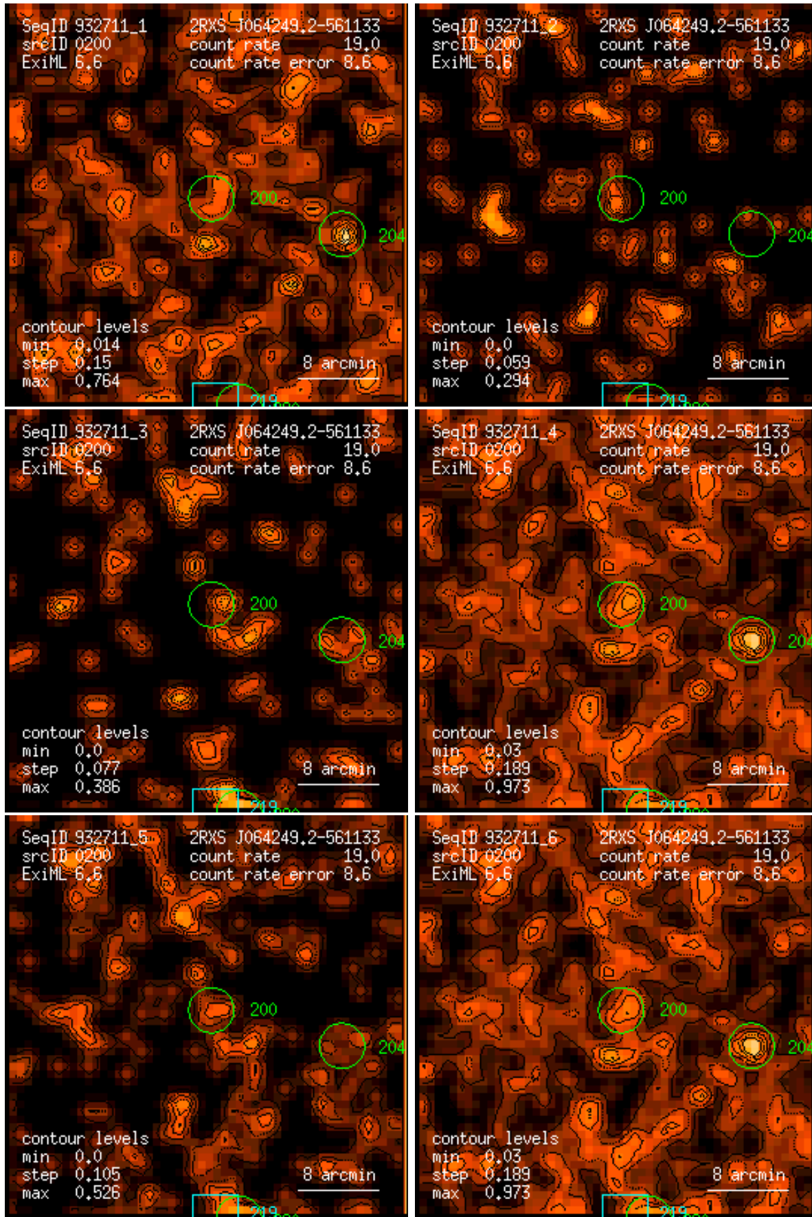
Figure 200: RASS 932711: detection 0200: band rate images, Gaussian filter: (1) PSPC channels 11 – 41, (2) 52 – 90, (3) 91 – 201, (4) 11 – 235, (5) 52 – 201, (6) 11 – 201. Broad band rates in counts/ks. Band rate contour levels in counts/ks/arcmin 2 .
