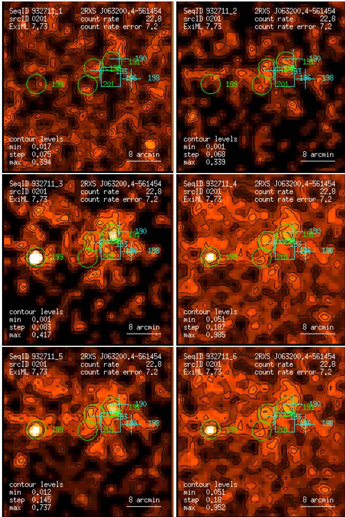
Figure 201: RASS 932711: detection 0201: band rate images, Gaussian filter: (1) PSPC channels 11 – 41, (2) 52 – 90, (3) 91 – 201, (4) 11 – 235, (5) 52 – 201, (6) 11 – 201. Broad band rates in counts/ks. Band rate contour levels in counts/ks/arcmin 2 .
