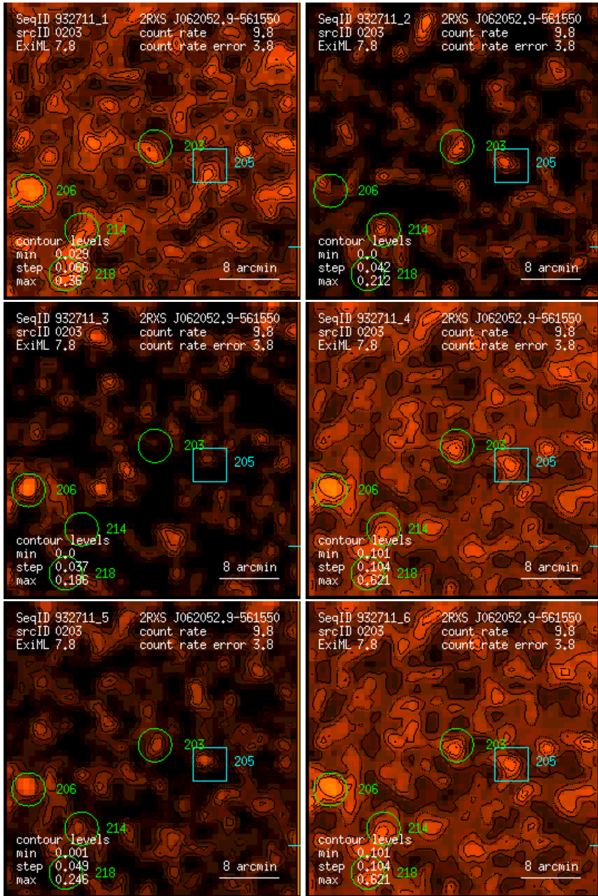
Figure 203: RASS 932711: detection 0203: band rate images, Gaussian filter: (1) PSPC channels 11 – 41, (2) 52 – 90, (3) 91 – 201, (4) 11 – 235, (5) 52 – 201, (6) 11 – 201. Broad band rates in counts/ks. Band rate contour levels in counts/ks/arcmin 2 .
