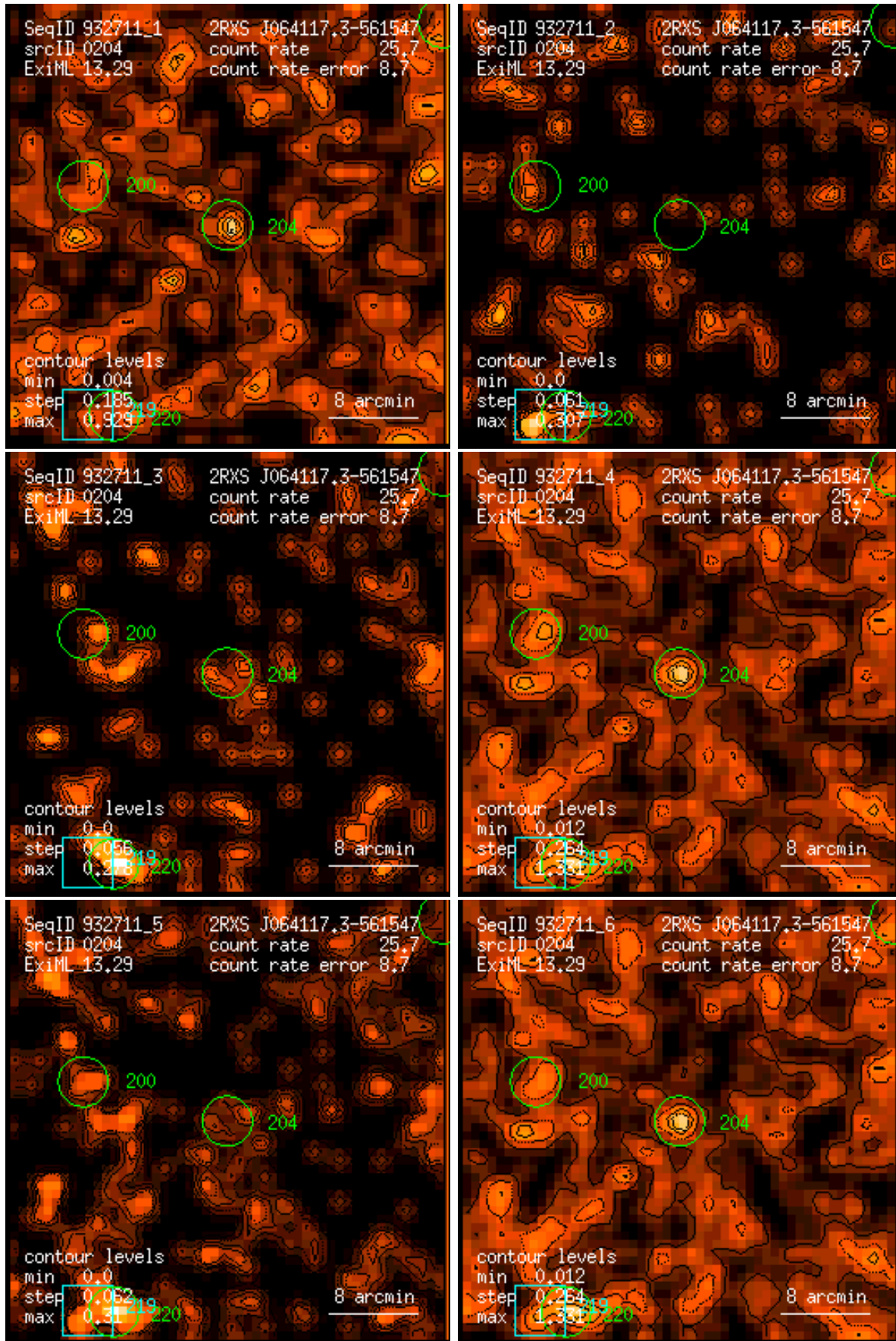
Figure 204: RASS 932711: detection 0204: band rate images, Gaussian filter: (1) PSPC channels 11 – 41, (2) 52 – 90, (3) 91 – 201, (4) 11 – 235, (5) 52 – 201, (6) 11 – 201. Broad band rates in counts/ks. Band rate contour levels in counts/ks/arcmin 2 .
