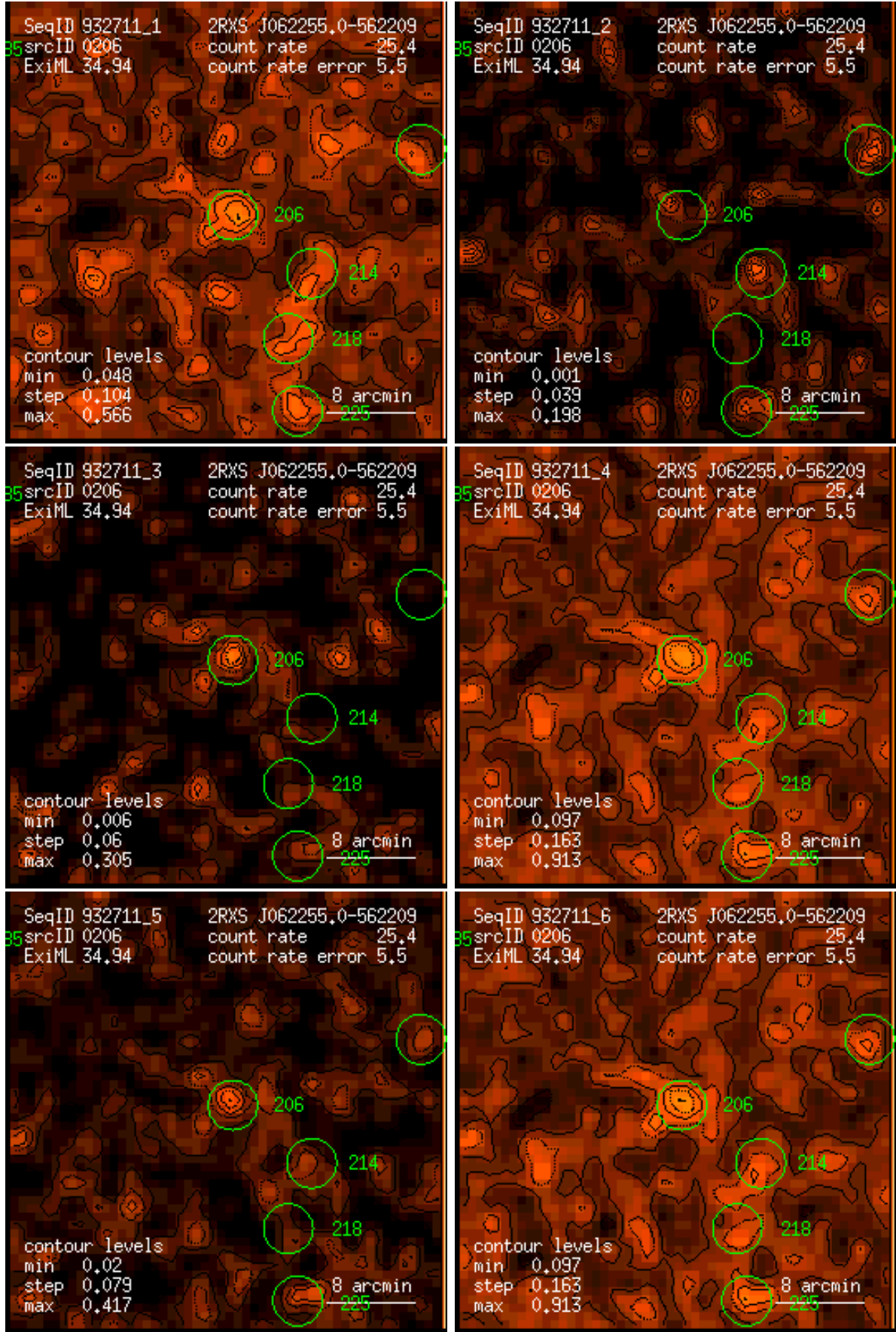
Figure 206: RASS 932711: detection 0206: band rate images, Gaussian filter: (1) PSPC channels 11 – 41, (2) 52 – 90, (3) 91 – 201, (4) 11 – 235, (5) 52 – 201, (6) 11 – 201. Broad band rates in counts/ks. Band rate contour levels in counts/ks/arcmin 2 .
