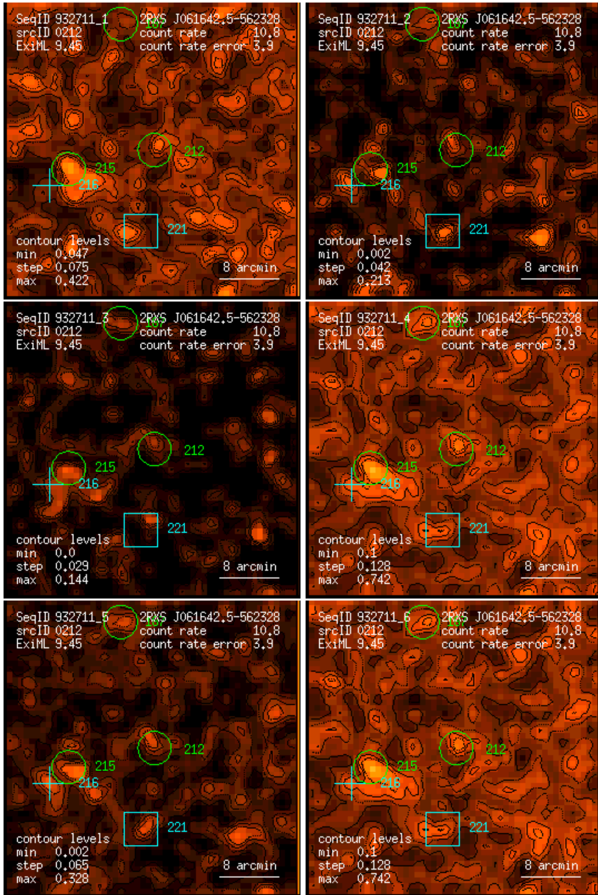
Figure 212: RASS 932711: detection 0212: band rate images, Gaussian filter: (1) PSPC channels 11 – 41, (2) 52 – 90, (3) 91 – 201, (4) 11 – 235, (5) 52 – 201, (6) 11 – 201. Broad band rates in counts/ks. Band rate contour levels in counts/ks/arcmin 2 .
