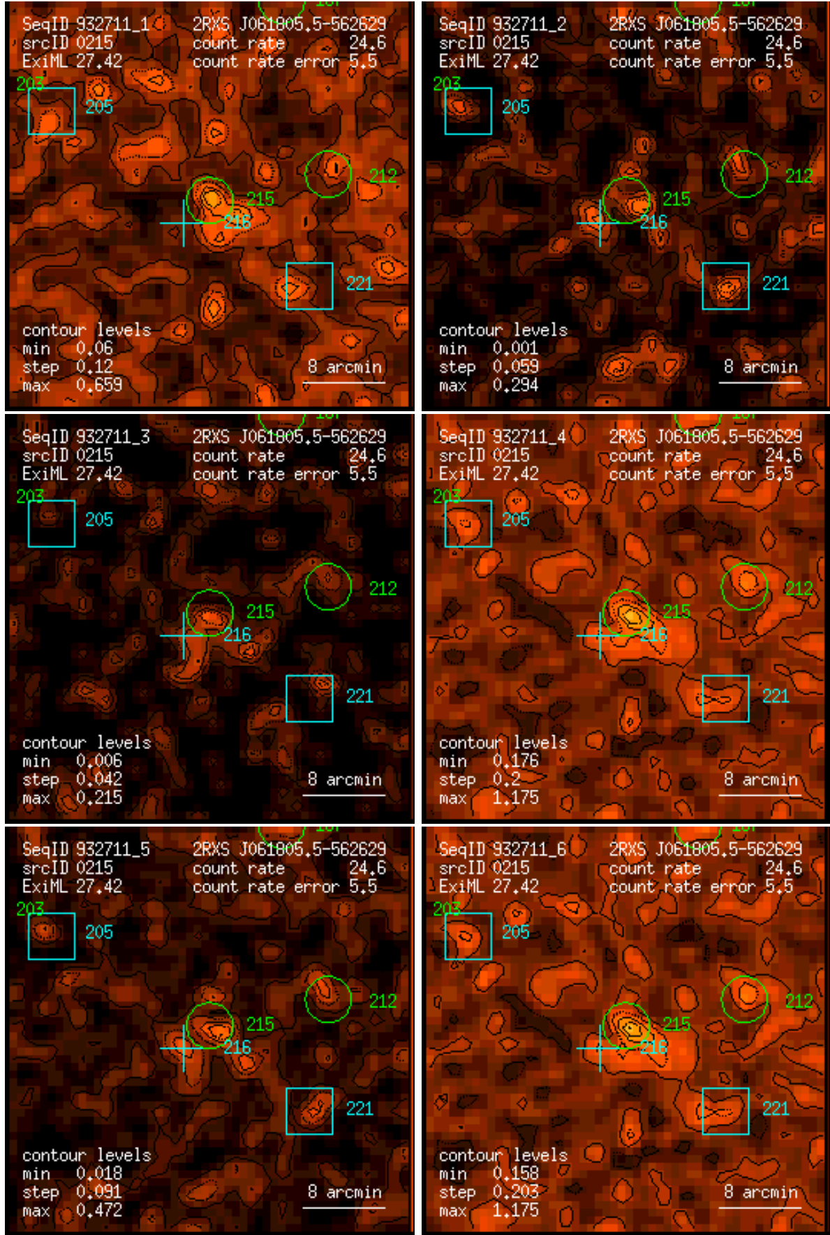
Figure 215: RASS 932711: detection 0215: band rate images, Gaussian filter: (1) PSPC channels 11 – 41, (2) 52 – 90, (3) 91 – 201, (4) 11 – 235, (5) 52 – 201, (6) 11 – 201. Broad band rates in counts/ks. Band rate contour levels in counts/ks/arcmin 2 .
