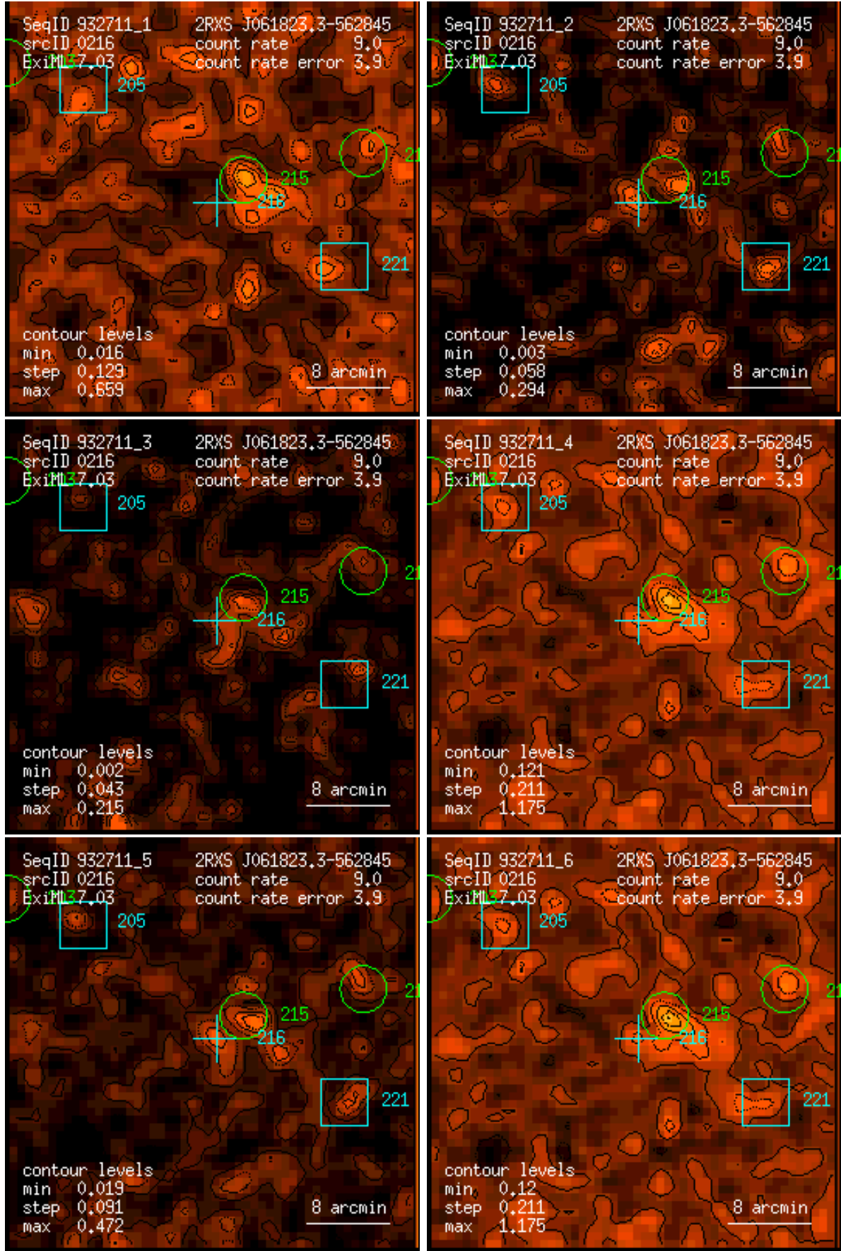
Figure 216: RASS 932711: detection 0216: band rate images, Gaussian filter: (1) PSPC channels 11 – 41, (2) 52 – 90, (3) 91 – 201, (4) 11 – 235, (5) 52 – 201, (6) 11 – 201. Broad band rates in counts/ks. Band rate contour levels in counts/ks/arcmin 2 .
