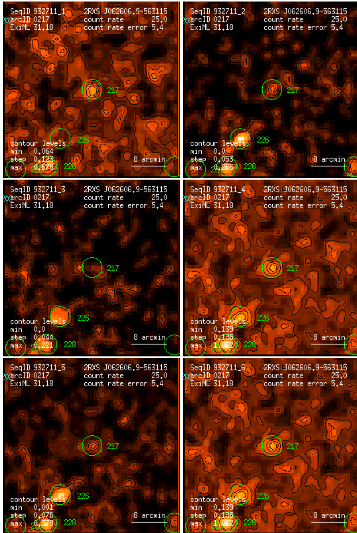
Figure 217: RASS 932711: detection 0217: band rate images, Gaussian filter: (1) PSPC channels 11 – 41, (2) 52 – 90, (3) 91 – 201, (4) 11 – 235, (5) 52 – 201, (6) 11 – 201. Broad band rates in counts/ks. Band rate contour levels in counts/ks/arcmin 2 .
