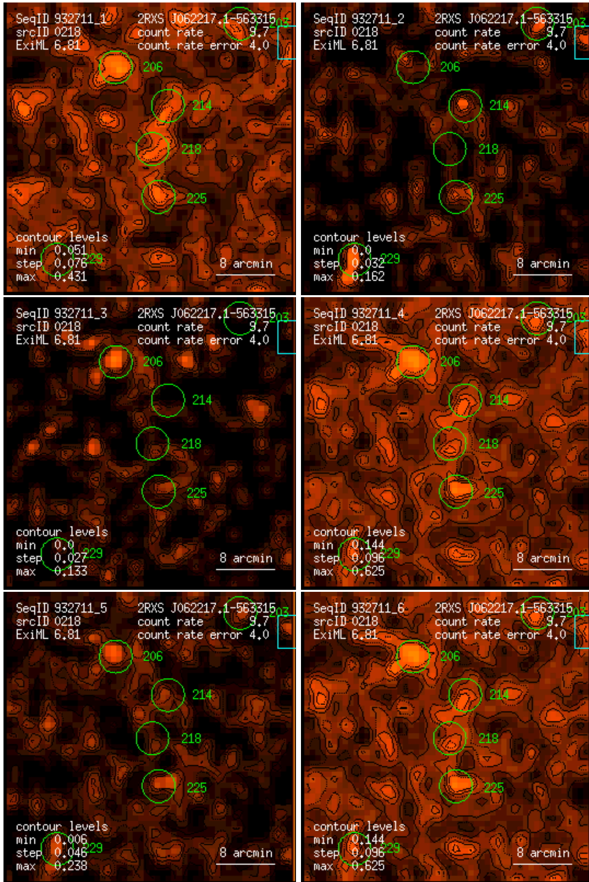
Figure 218: RASS 932711: detection 0218: band rate images, Gaussian filter: (1) PSPC channels 11 – 41, (2) 52 – 90, (3) 91 – 201, (4) 11 – 235, (5) 52 – 201, (6) 11 – 201. Broad band rates in counts/ks. Band rate contour levels in counts/ks/arcmin 2 .
