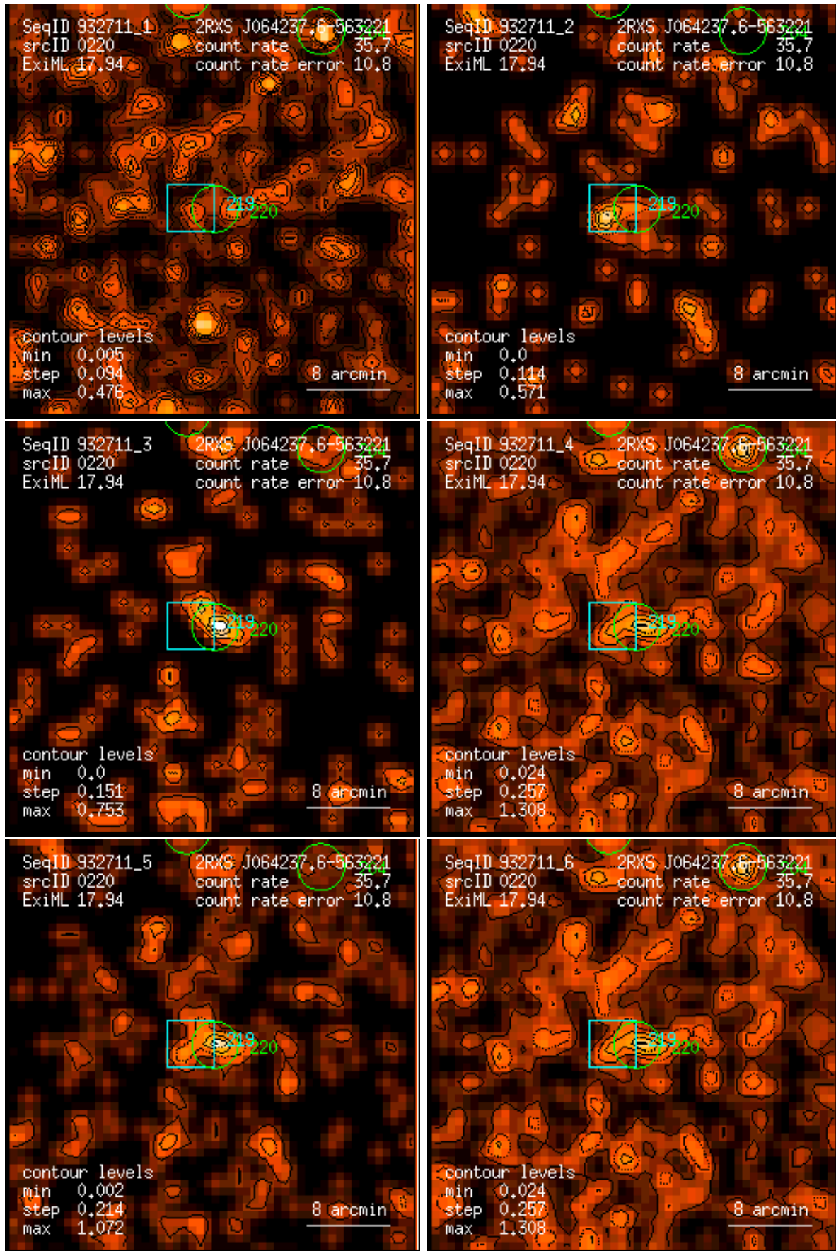
Figure 220: RASS 932711: detection 0220: band rate images, Gaussian filter: (1) PSPC channels 11 – 41, (2) 52 – 90, (3) 91 – 201, (4) 11 – 235, (5) 52 – 201, (6) 11 – 201. Broad band rates in counts/ks. Band rate contour levels in counts/ks/arcmin 2 .
